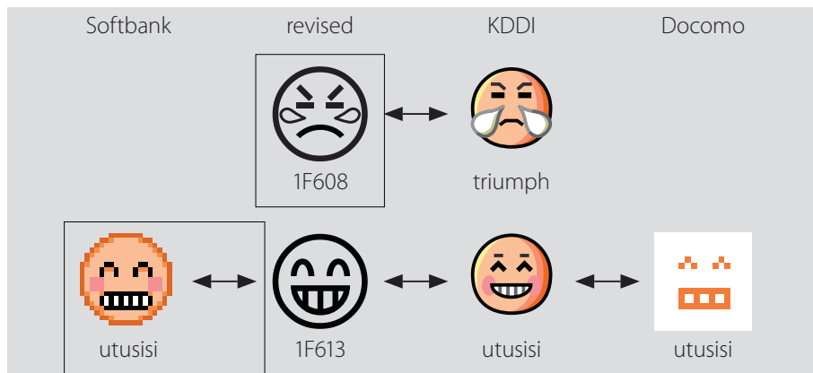
fig. 5: Revised mappings and glyphs
