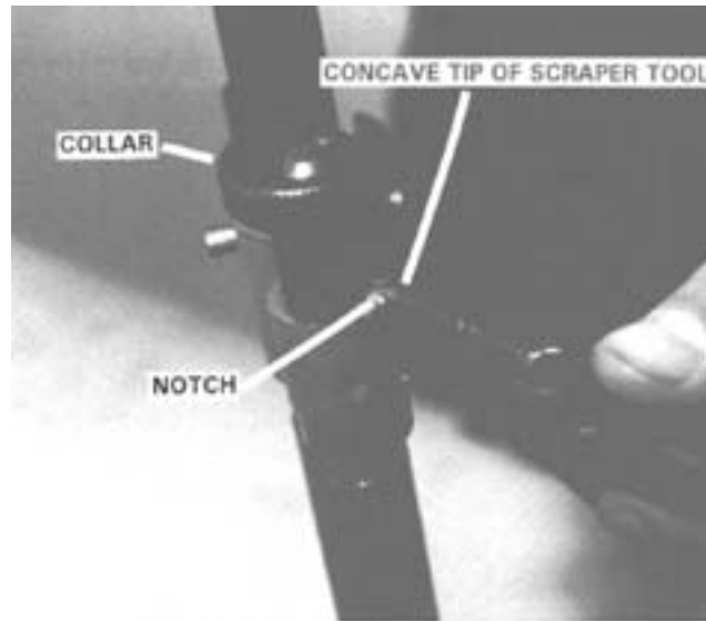
Step 1. Placement of the Scraper Tool.
