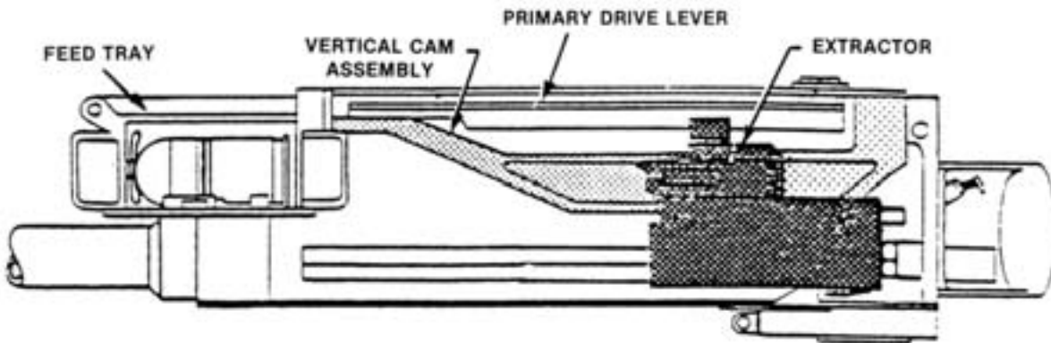
Figure 5-24. Round Positioned In Feeder, Bolt to Rear.
