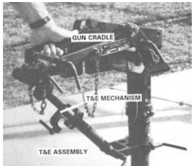
Figure 4-72. M4 Pedestal Mount With MK64 MOD 5 Cradle.
