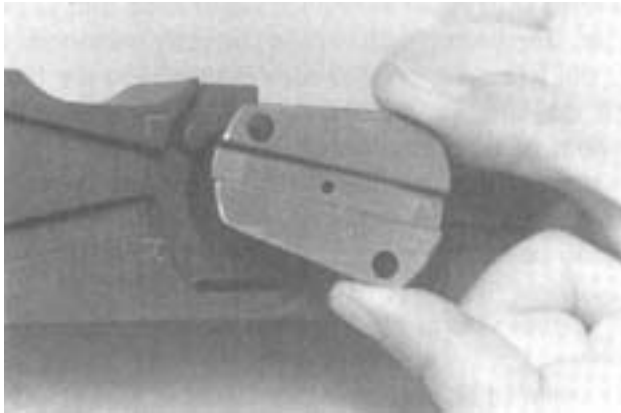
Figure 4-33. Replacing the Bolt Switch and Stud.
