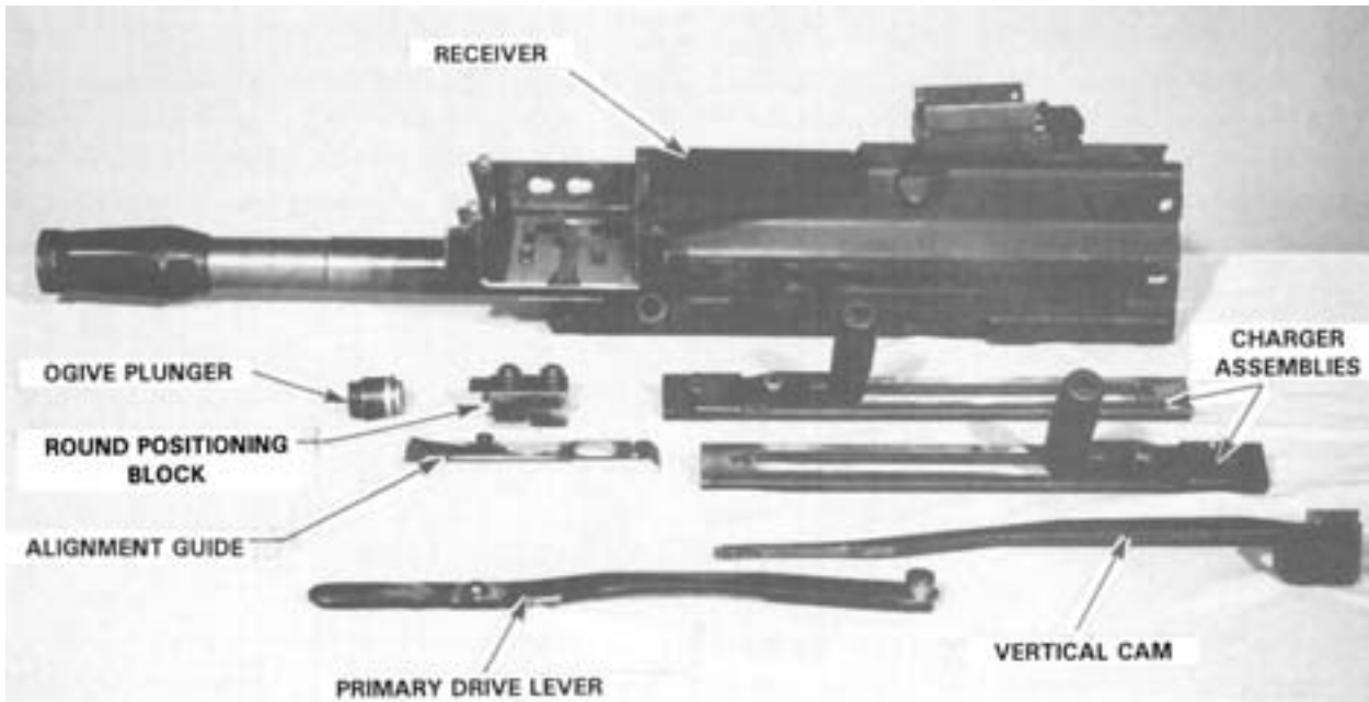
Figure 5-16. Receiver Assembly, Detailed Disassembled.
