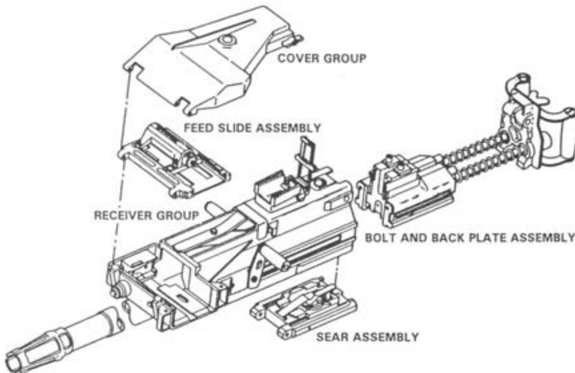
Figure 5-5. Five Main Groups, Exploded View.
