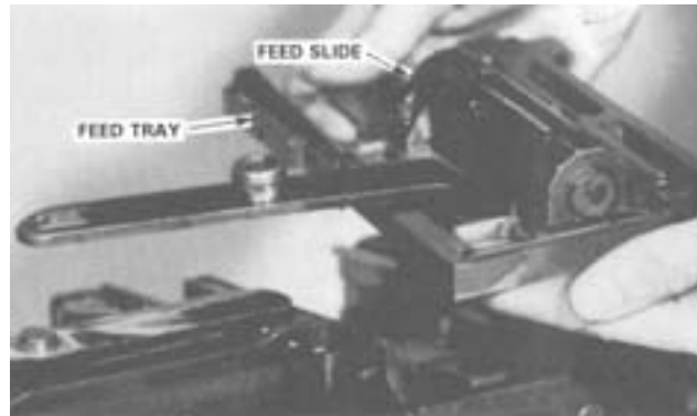
Figure 5-11. Removing the Feed Slide Assembly.
