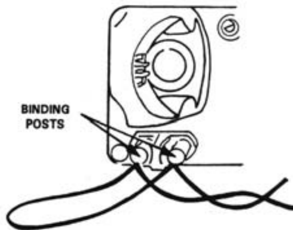
Figure 6-74. Connection of the Wire Loop.
