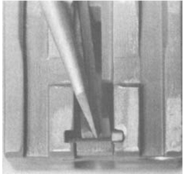
Figure 4-23. Prying the Sear Stop into the Center Recess.
