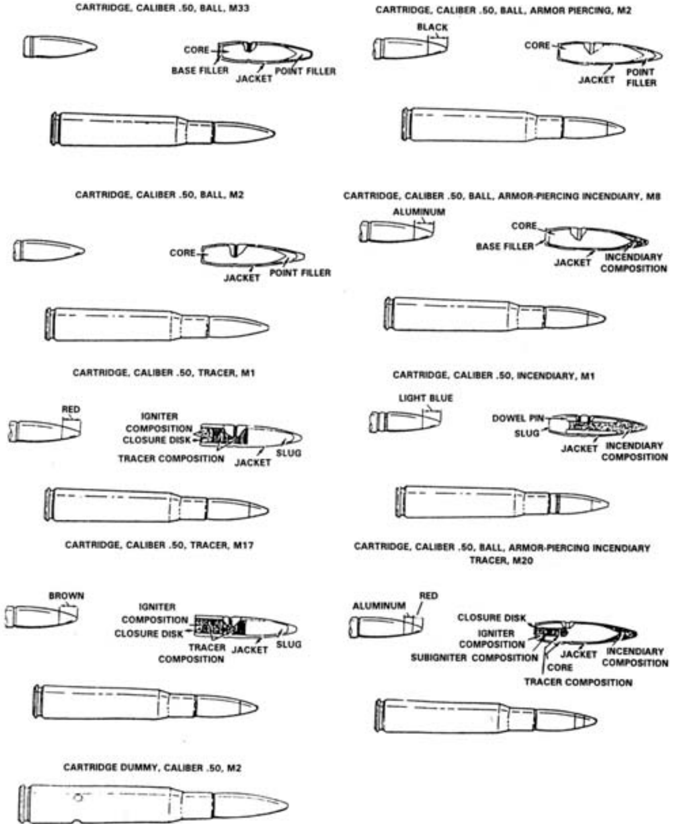
Figure 4-82. M2 .50 Cal Ammunition.
