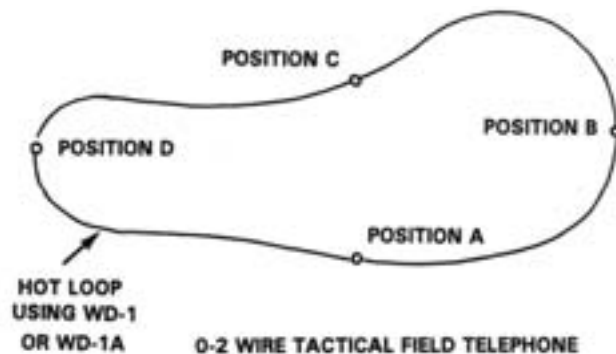
Figure 6-73. Installation of the Wire Loop.
