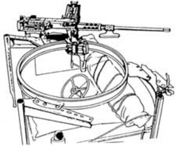
Figure 4-73. M66 Truck Ring Mount.
