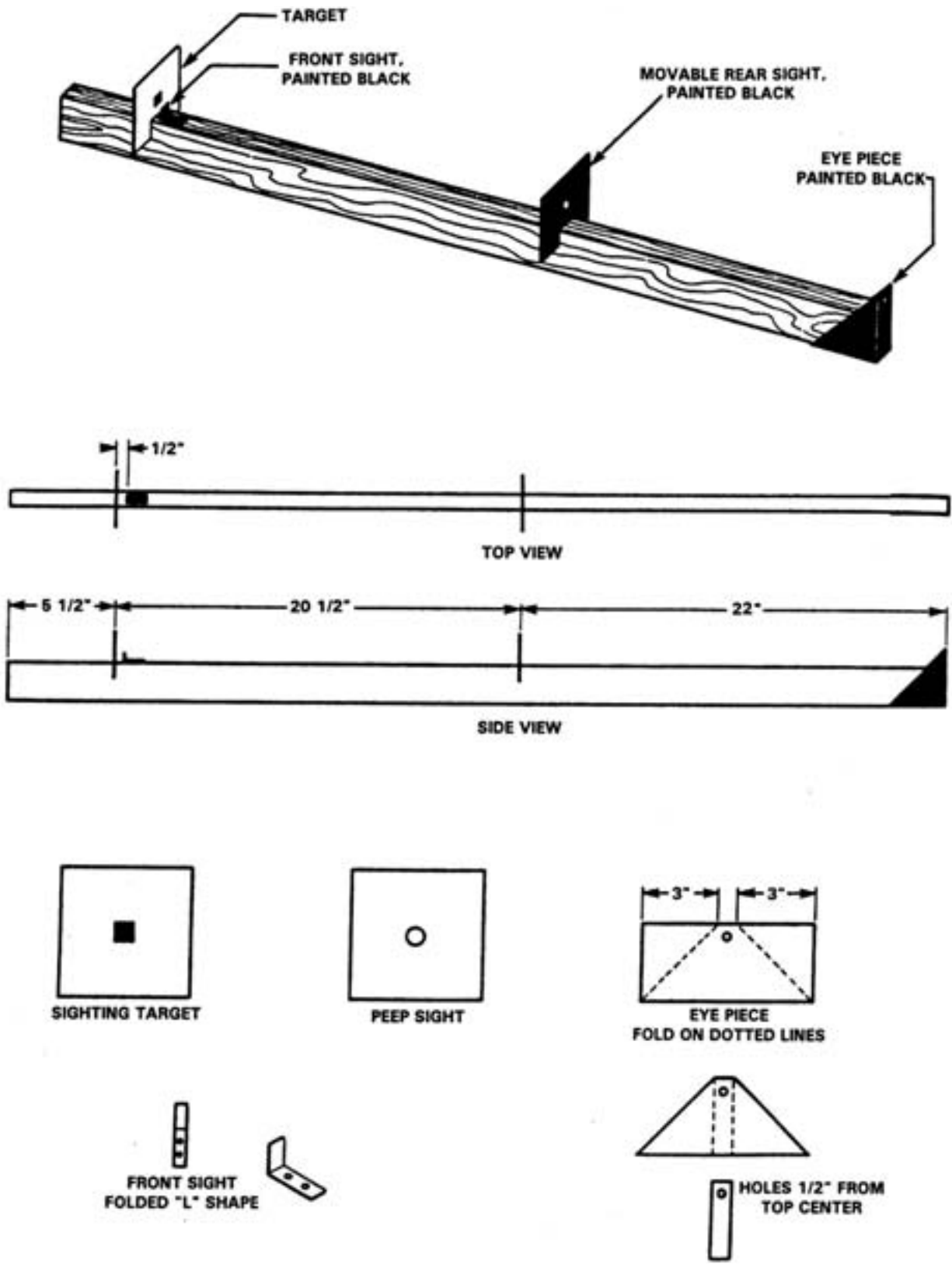
Figure 4-107. Sighting Bar.
