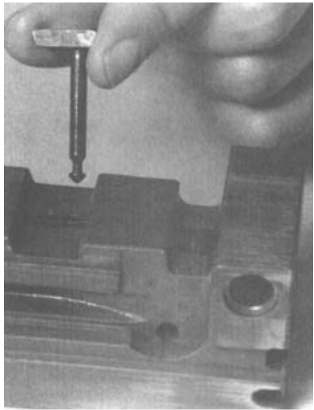
Figure 4-25. Drifting the Sear Stop Pin Free From Engagement with the Firing Pin Spring.
