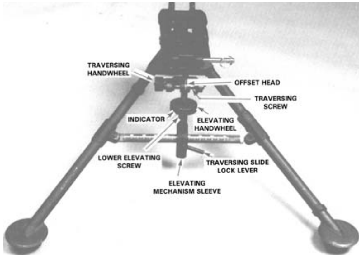
Figure 3-41. T&E Mechanism.
