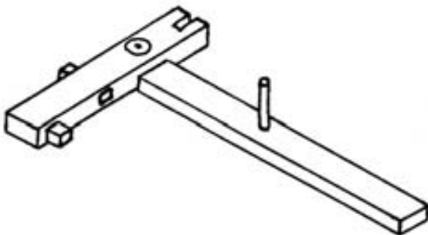
Figure 3-72. Combination Front Sight Adjusting Tool.
