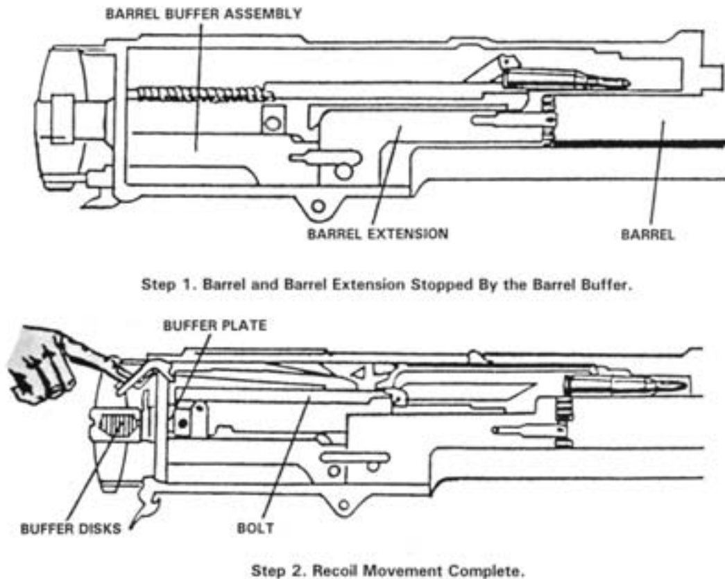
Figure 4-65. Unlocking.
