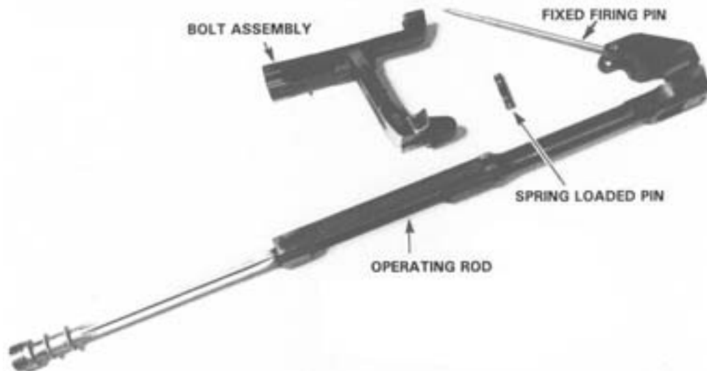
Figure 3-15. Operating Group, Detailed Disassembly.
