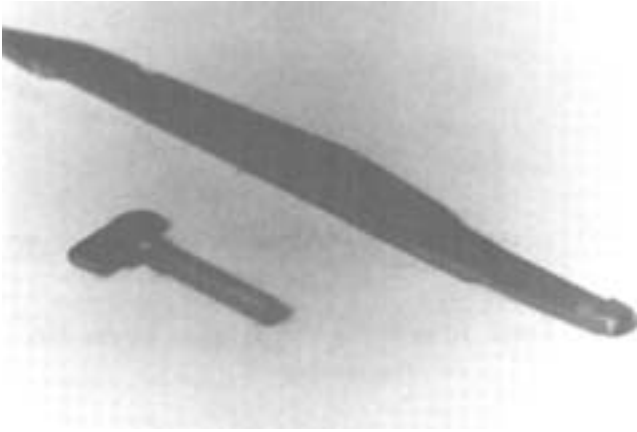
Figure 4-50. Trigger Lever and Trigger Lever Pin Assemblies.
