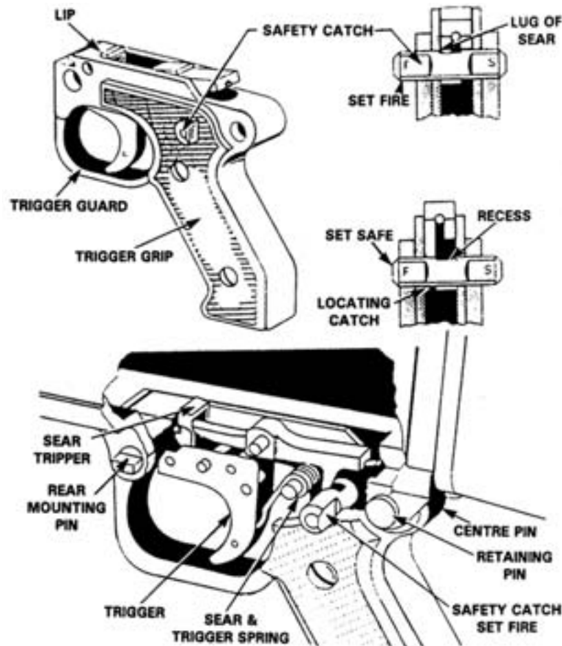
Figure 3-61. Operation of the Safety.
