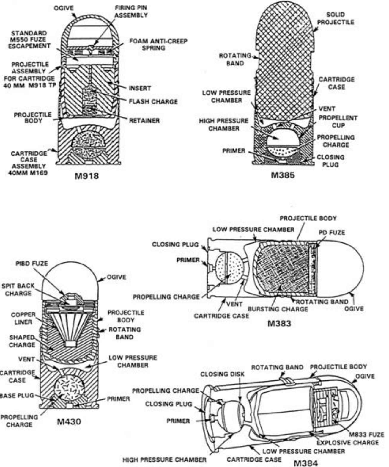
Figure 5-43. MK-19 40mm Ammunition—Continued.
