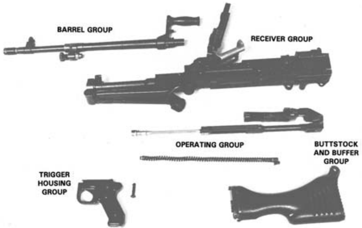
Figure 3-5. Five Main Groups.
