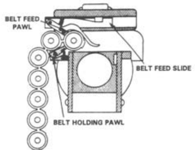
Figure 4-56. Feeding (Rear View).
