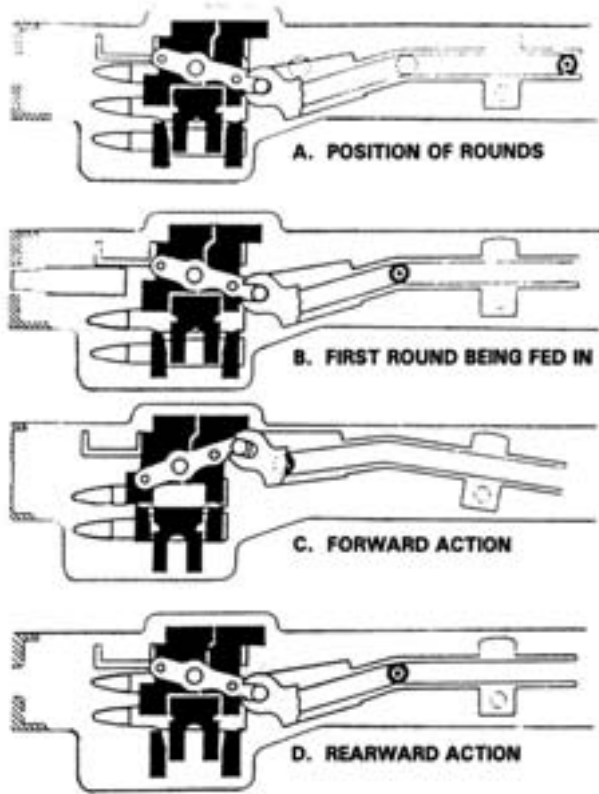
Figure 3-23. Feeding.
