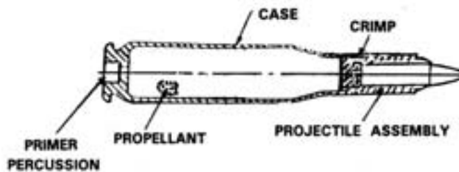
Figure 4-82. M2 .50 Cal Ammunition—Continued.
