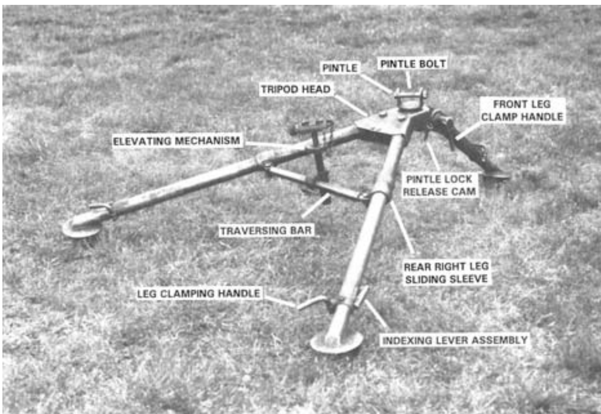
Figure 4-69. Tripod Mount, M3.
