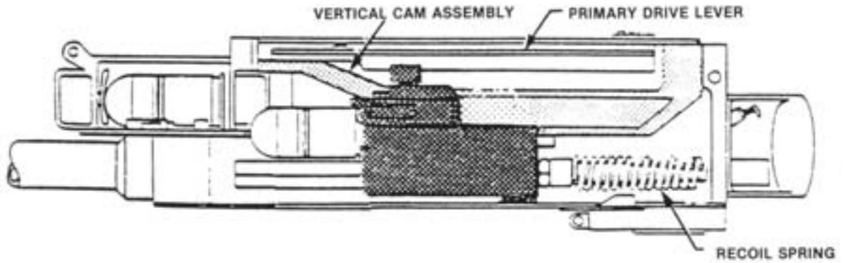
Figure 5-25. Round Picked Up by Extractors.
