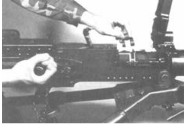
Figure 4-5. Aligning Barrel Locking Spring Lug With the 3/8-inch Hole.
