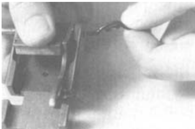
Figure 4-41. Drifting Out the Belt Feed Pawl Pin.
