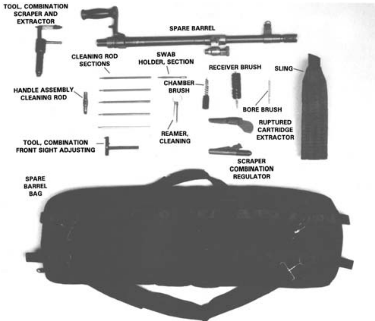
Figure 3-46. Spare Barrel Bag.
