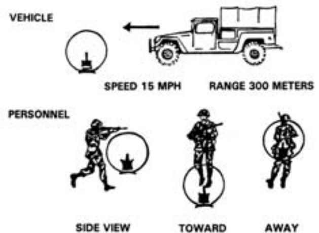
Figure 6-21. Moving Target Aiming Points.
