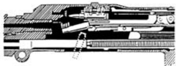
Figure 3-30. Extraction and Ejection.
