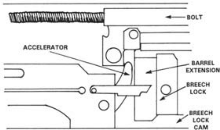
Figure 4-63. Locking.
