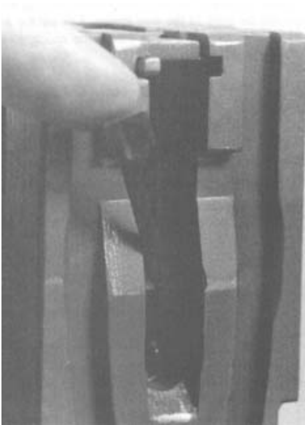
Figure 4-24. Prying the Accelerator Stop Lock into the Center Recess.
