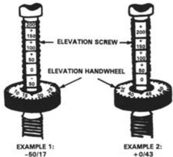
Figure 6-29. Elevation Reading.
