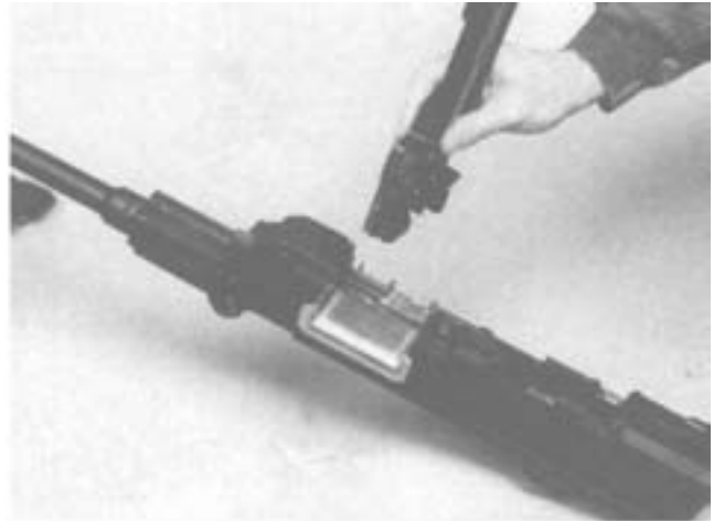
Step 2. Removing the Cover and Feed Tray.
