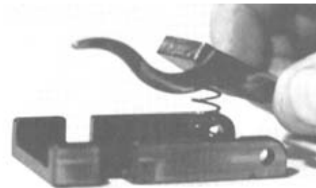
Figure 4-42. Removing the Belt Feed Pawl and Arm.
