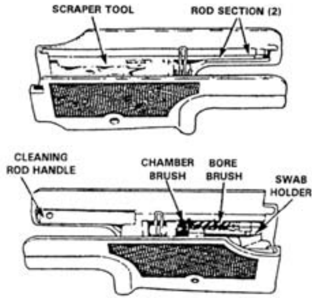
Figure 2-34. SAW Tool Storage.
