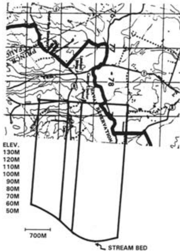
Figure 6-49. Sample Terrain Profile.
