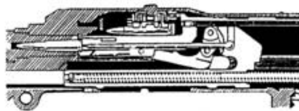
Figure 3-26. Locking.
