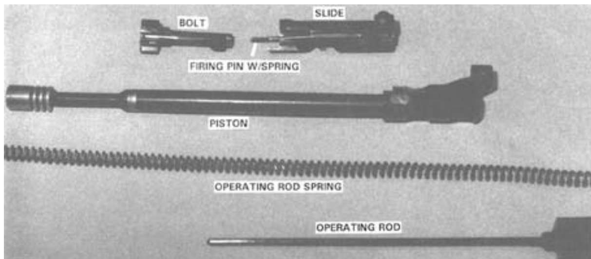
Figure 2-15. Operating Group, Detailed Disassembled.
