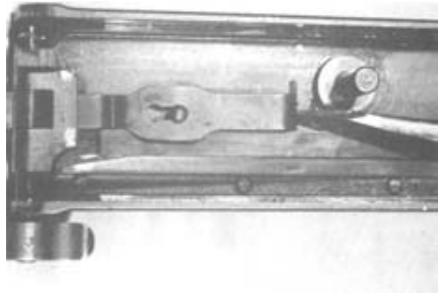
Figure 4-45. Replacing the Cover Latch Spring.
