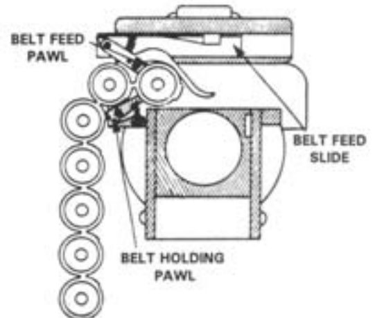
Figure 4-60. Belt Feed Pawl Behind the First Round.
