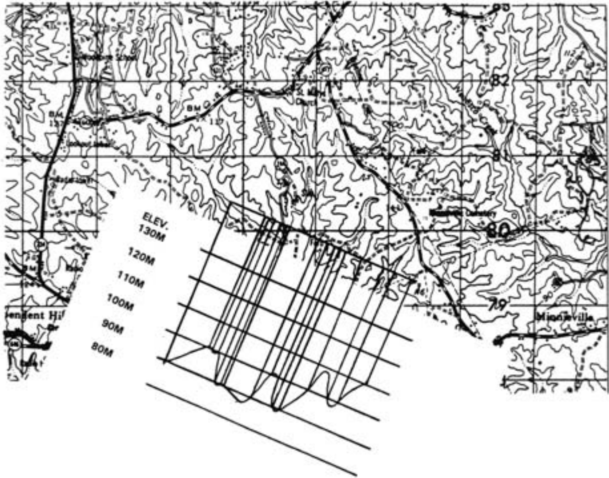
Figure 6-48. Terrain Profiling.
