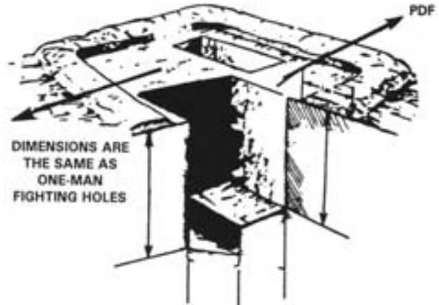
Figure 6-72. Two-Hole Machine Gun Position.
