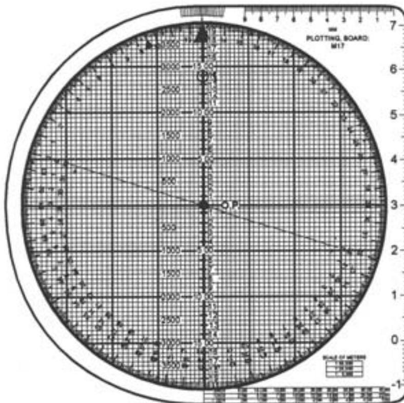
Figure F-3. GUN-TGT Azimuth (GUN-TGT Azimuth of 1400 Mils; Range 1,400 Meters).
