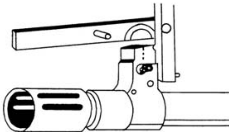
Figure 3-75. Unlocking the Front Sight Retaining Strap.
