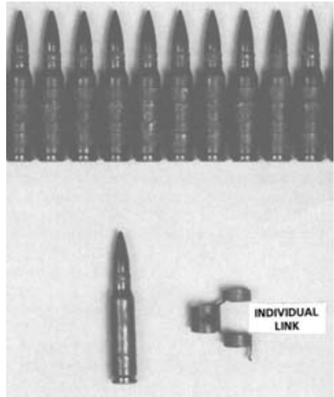
Figure 3-51. Belt of Disintegrating Link Ammunition.
