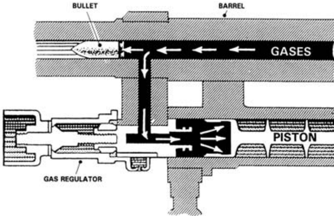
Figure 3-28. Action of the Gas.
