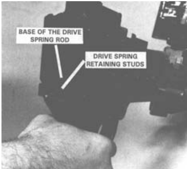
Step 1. Pushing In and Up on the Base of the Driving Spring Guide.
