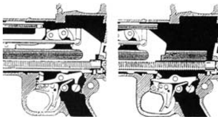
Figure 3-22. Trigger Pull Releasing the Operating Group.
