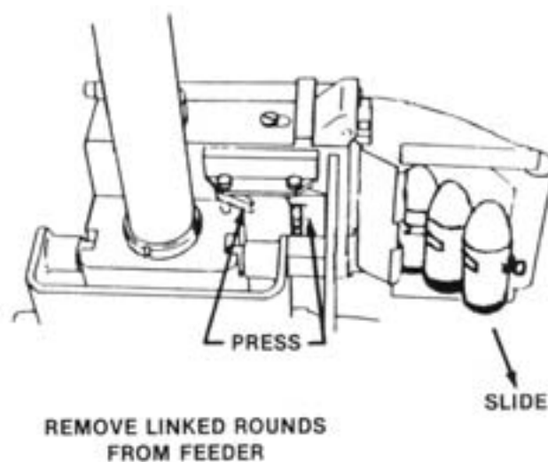
Figure 5-50. Clearing Rounds From Gun.
