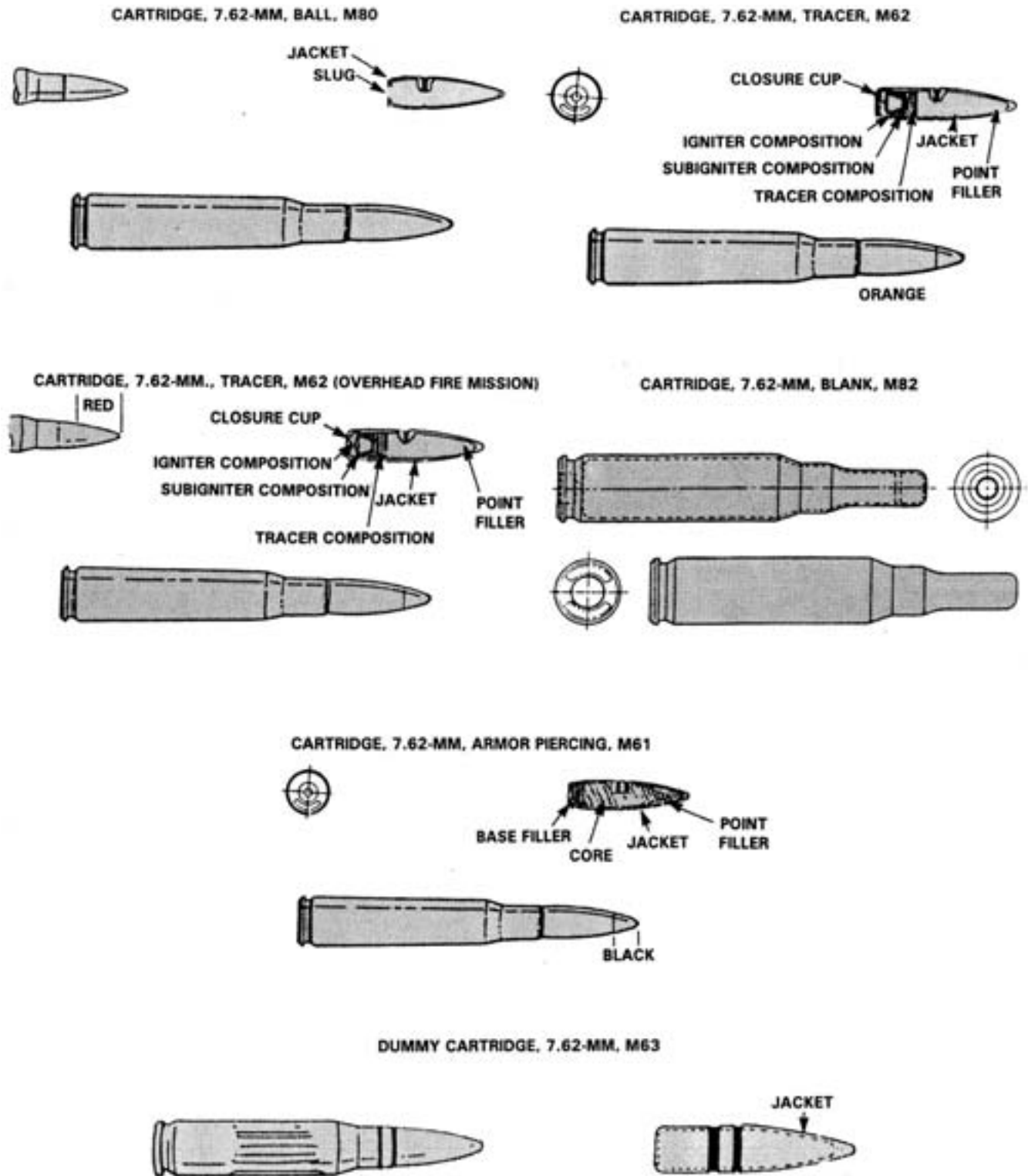
Figure 3-52. Ammunition for the M240G.
