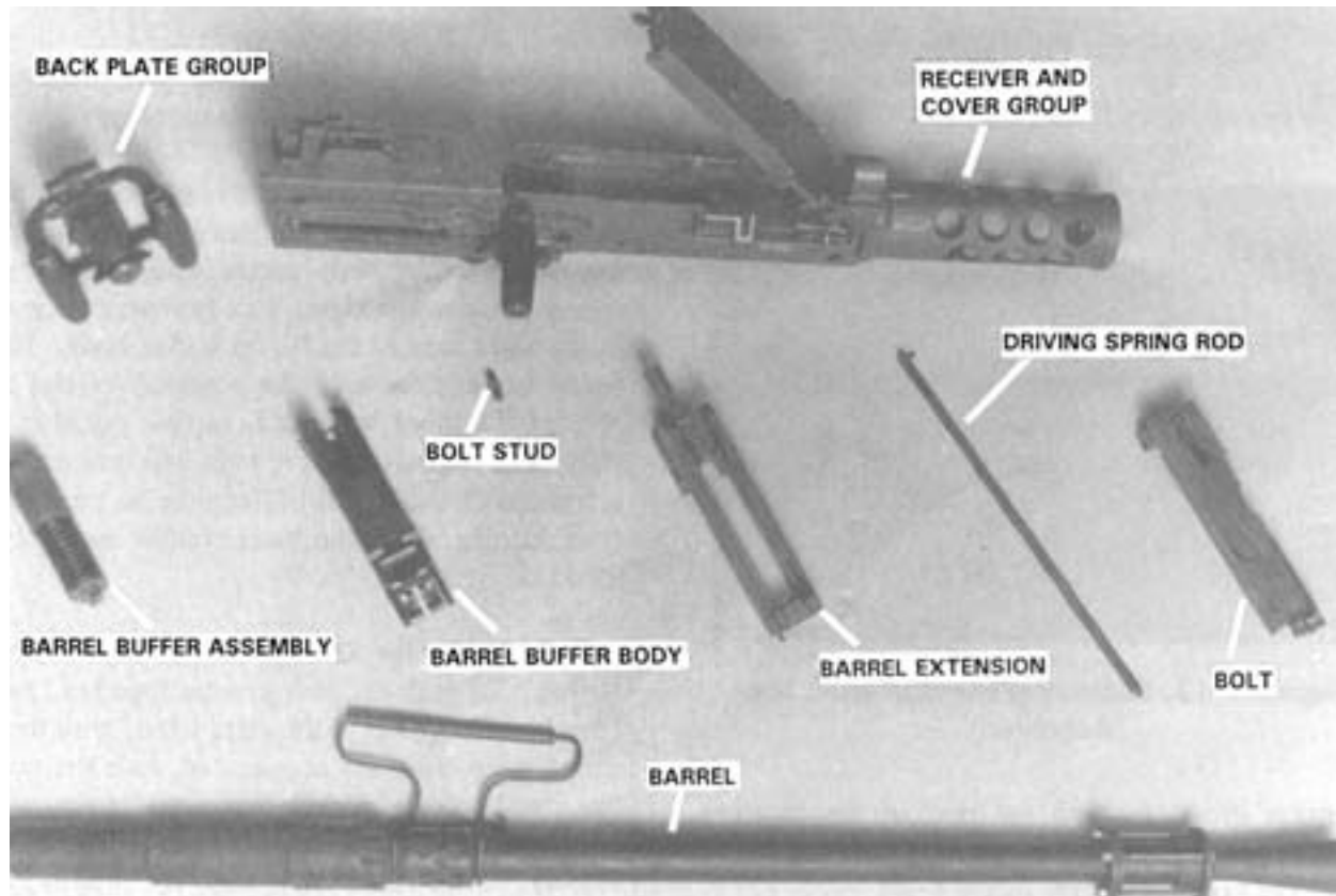
Figure 4-17. The Eight Major Groups and Assemblies.
