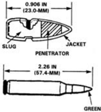
CARTRIDGE, 5.56MM, BALL, M855
