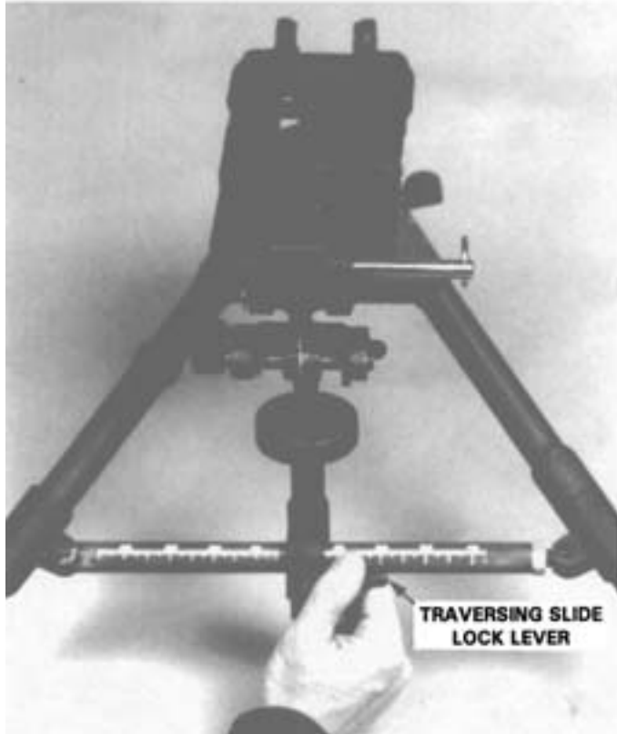
Figure 3-42. Attaching the Flex-mount to the Tripod—Continued.
