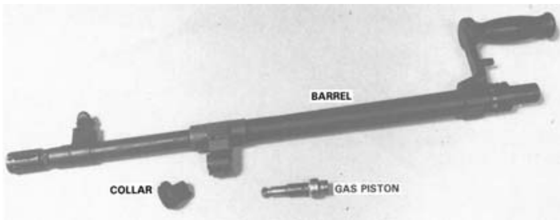
Figure 3-18. Barrel Group, Detailed Disassembly.
