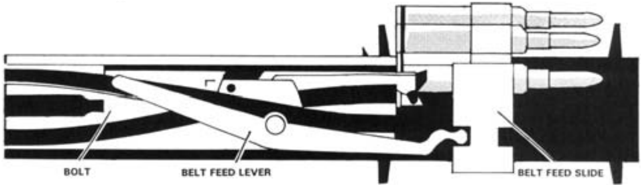
Figure 4-57. Feeding (Top View).
