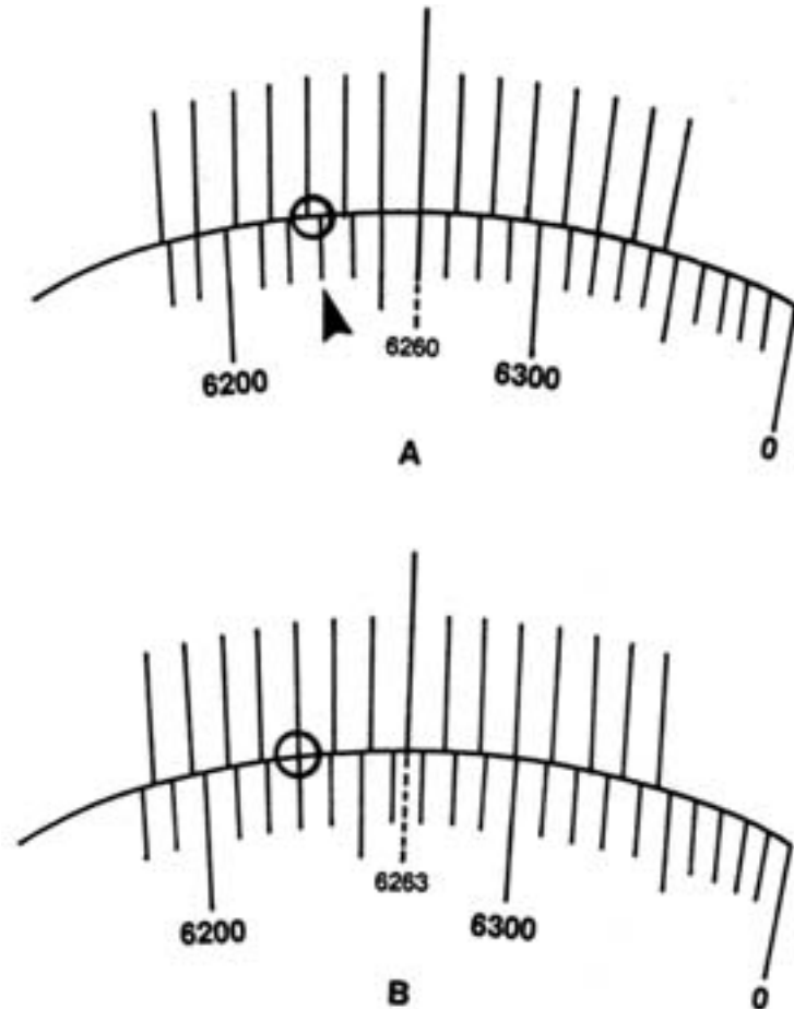
Figure E-3. Example of Use of Vernier Scale.
