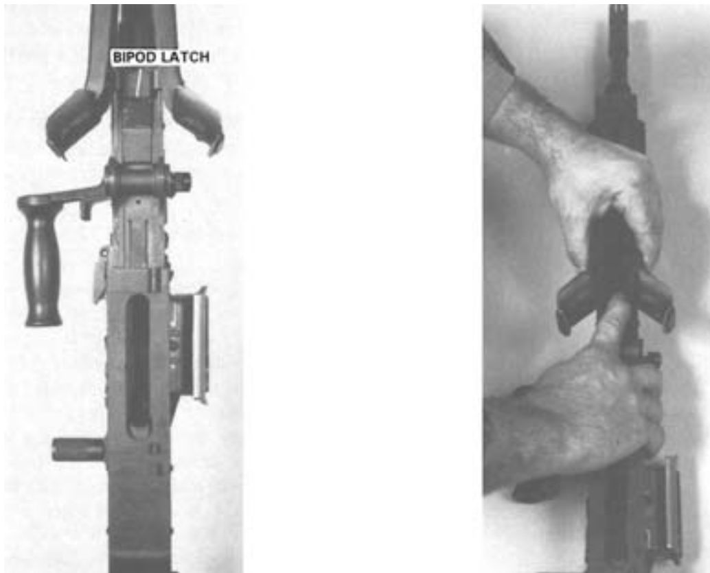
Figure 3-36. Lowering the Bipod.
