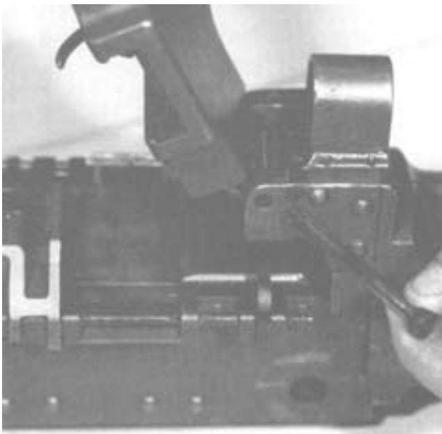
Figure 4-37. Removing the Cover Group.
