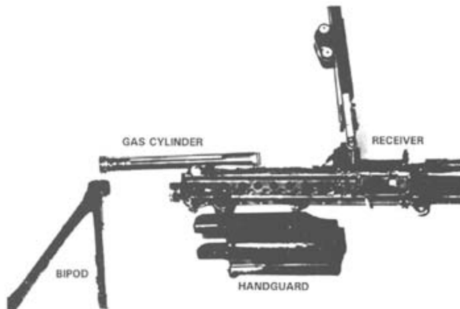
Figure 2-24. Receiver Group, Detail Disassembled.
