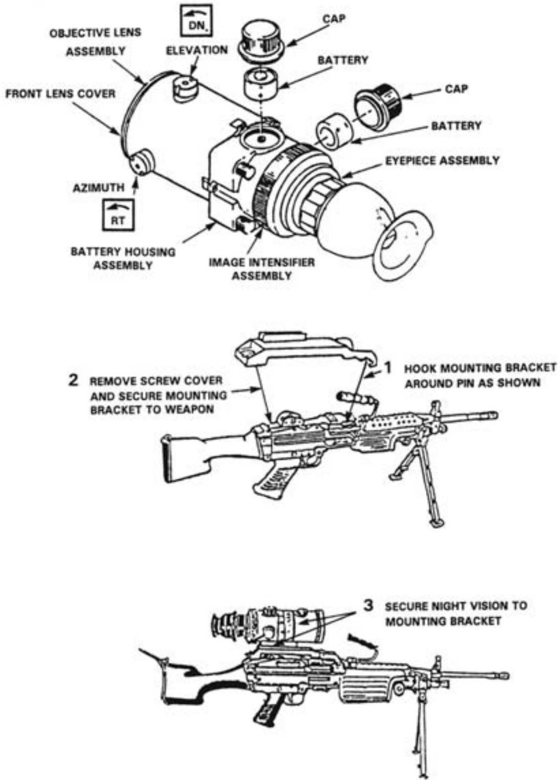
Figure 2-31. Mounting the Bracket and the Device.
