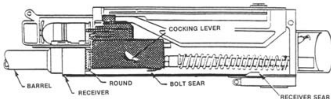
Figure 5-30. Firing/Unlocking.
