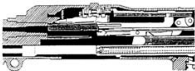
Figure 3-55. Firing From the Open Bolt Position.
