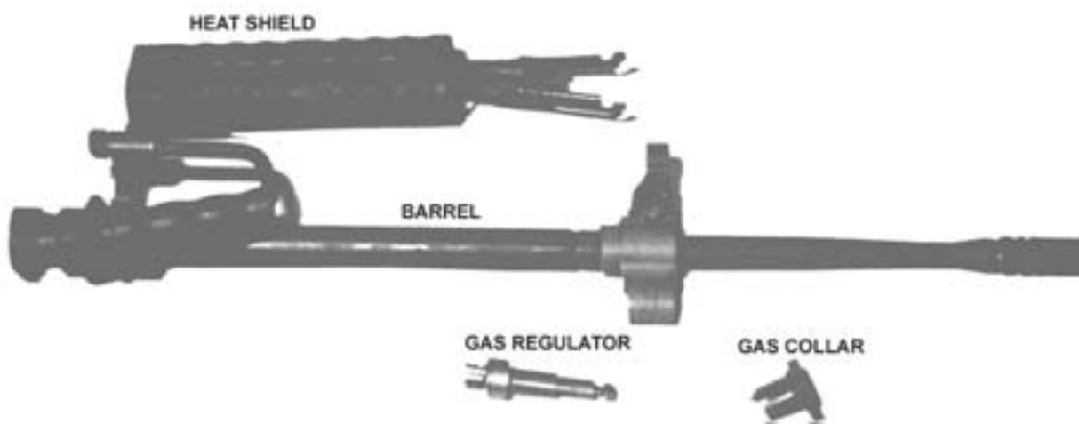
Figure 2-19. Barrel Group, Detail Disassembled.
