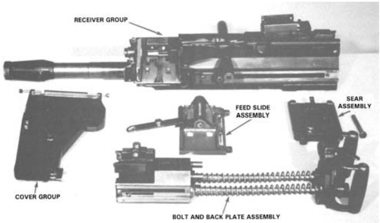
Figure 5-6. Five Main Groups.
