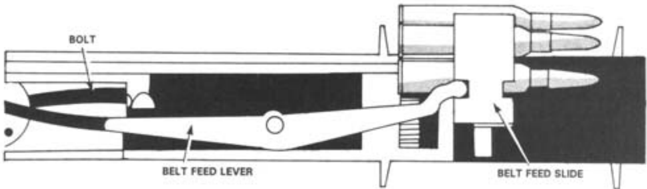
Figure 4-58. Belt Feed Slide Moving Out of the Side of the Cover.
