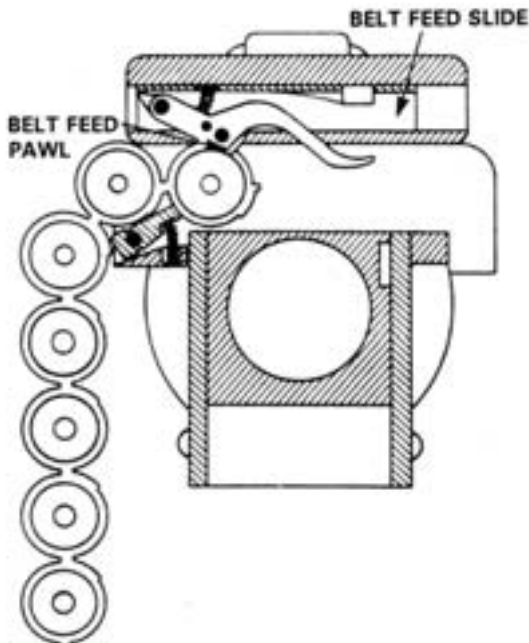
Figure 4-59. Belt Feed Pawl Riding Over the First Round
