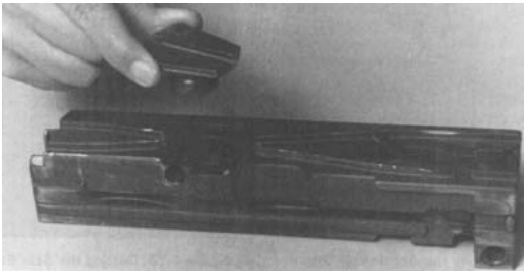
Figure 4-21. Removing the Bolt Switch and Bolt Switch Stud.
