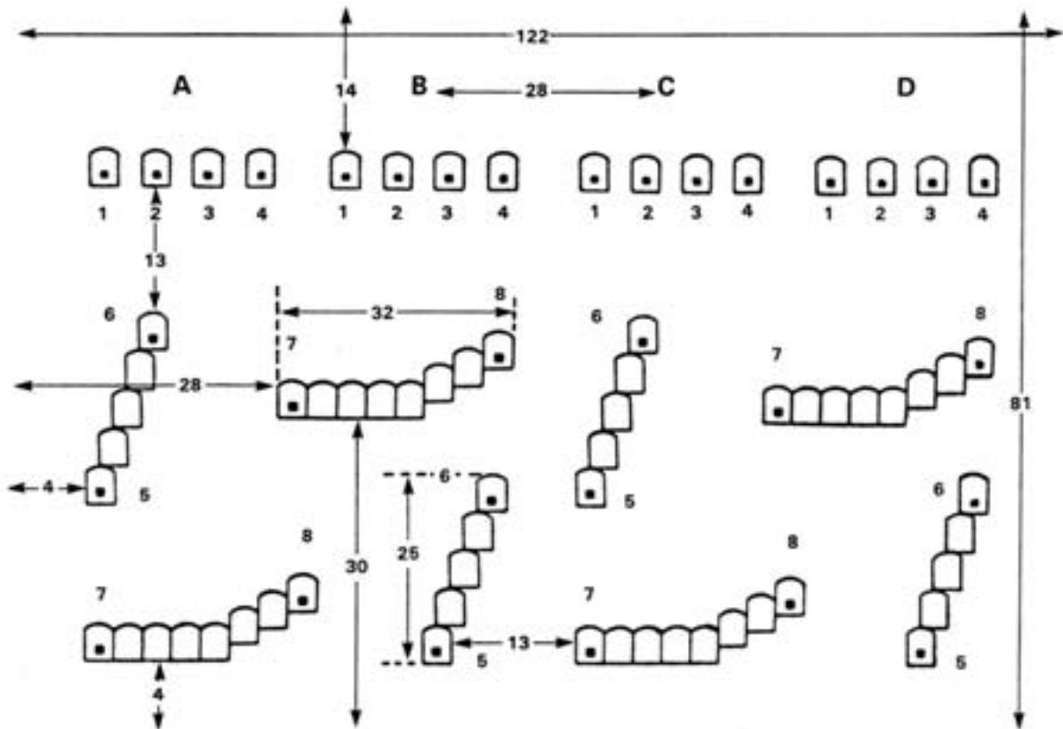
Figure 4-108. M2 .50 Cal Targets.
