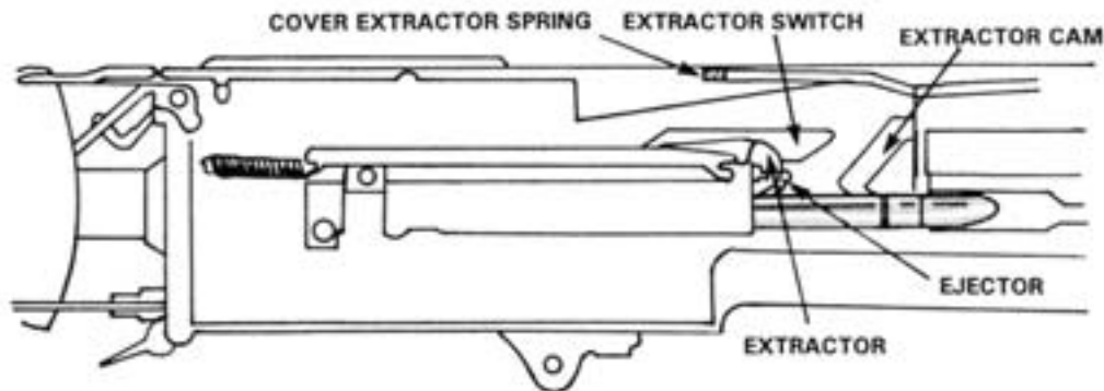
Figure 4-62. Chambering.
