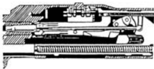
Figure 3-29. Unlocking.
