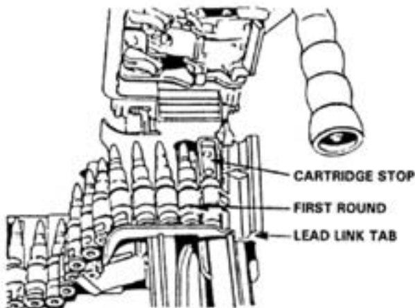
Figure 2-42. Cartridges in Metallic Belt.
