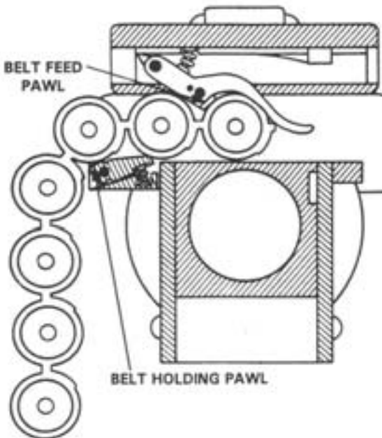
Figure 4-61. Belt Feed Slide Moving Inside the Cover.
