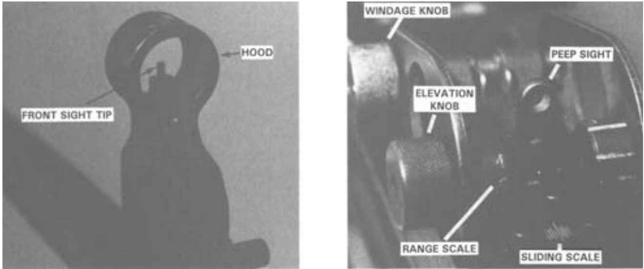
Figure 2-2. Front and Rear Sights.
