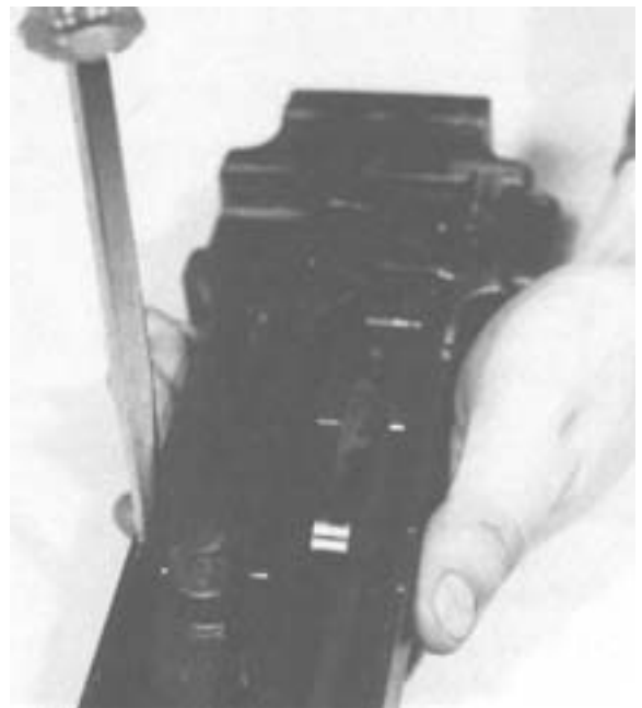
Figure 4-38. Removing the Belt Feed Lever.
