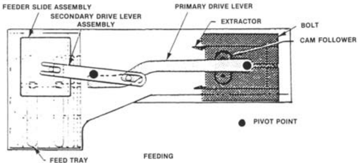
Figure 5-23. Position of Drive Levers, Bolt to Rear.
