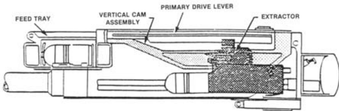
Figure 5-26. Round Cammed Down Onto Face of Bolt.
