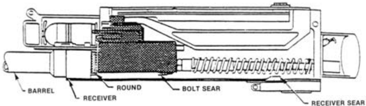
Figure 5-29. Chambering/Locking.
