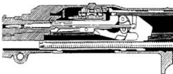
Figure 3-27. Firing.
