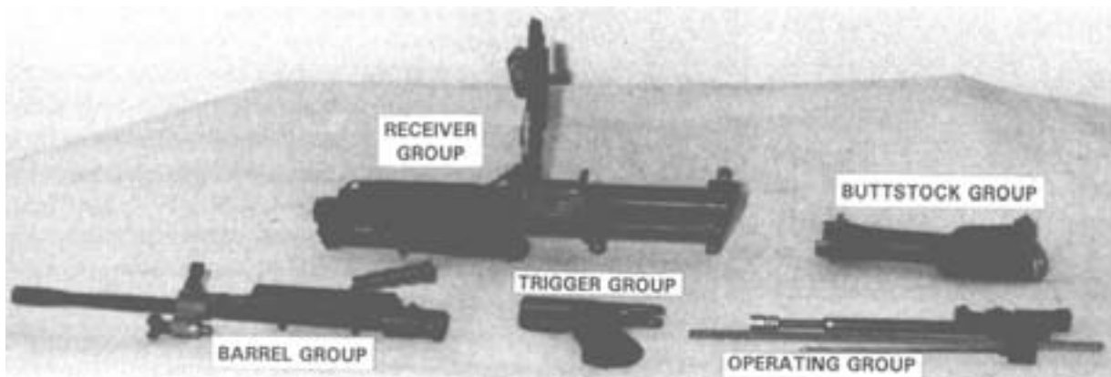
Figure 2-4. Five Main Groups (General Assembly).
