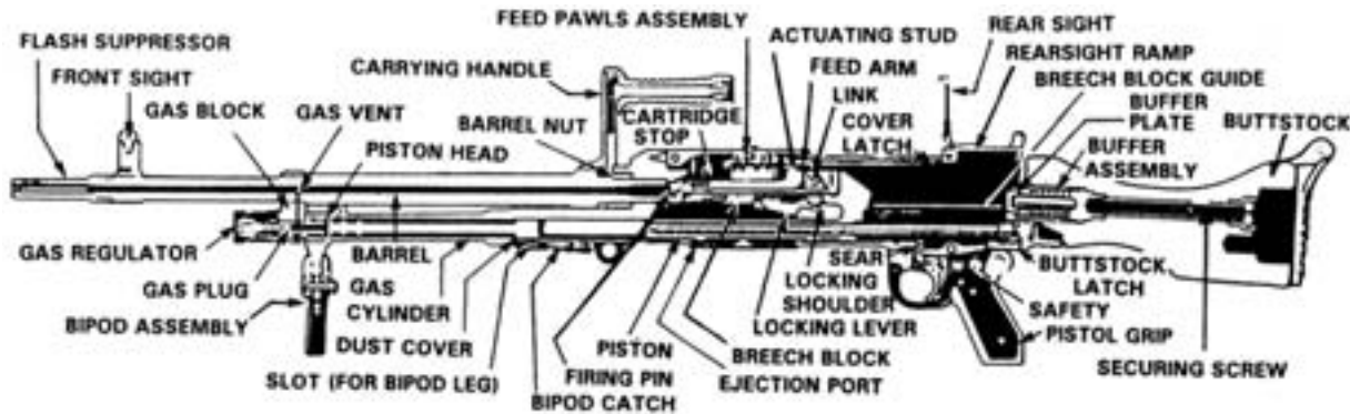
Figure 3-4. Cutaway View.
