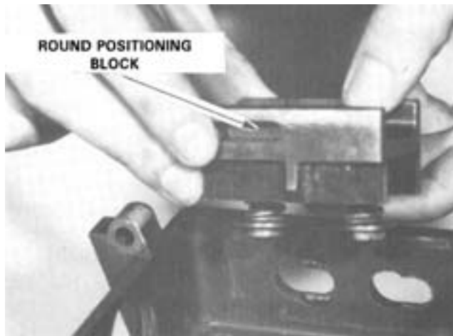
Figure 5-21. Removing of Round Positioning Block.
