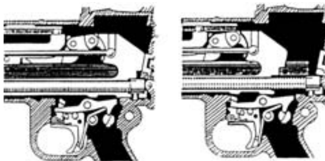
Figure 3-31. Cocking.
