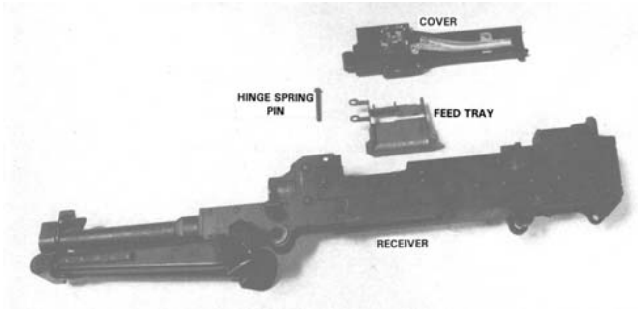
Figure 3-20. Receiver Group, Detailed Disassembly.
