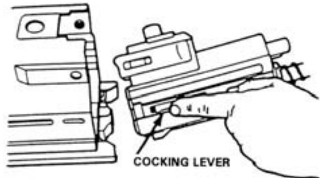
Figure 5-14. Inserting the Bolt and Backplate Assembly Into Receiver.
