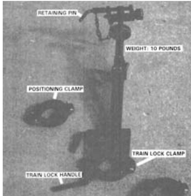
Figure 5-41. T&E Mechanism Mount Assembly.
