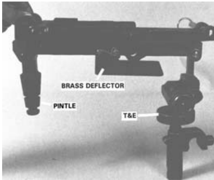
Figure 3-40. Flex-mount.
