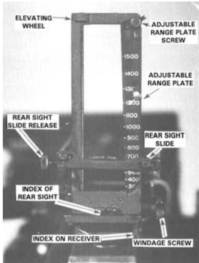
Figure 5-3. Rear Sight.
