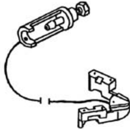
Figure 3-76. Blank Firing Adapter Assembly.
