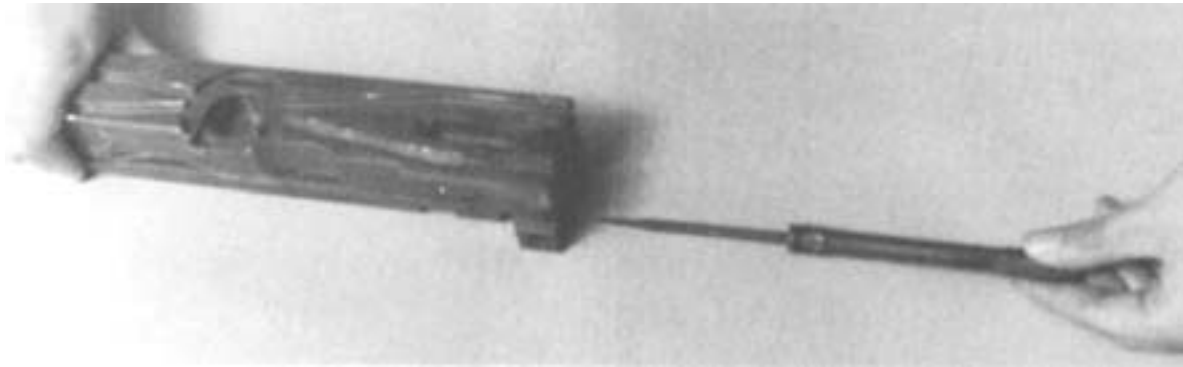
Figure 4-31. Replacing the Firing Pin and Extension Assembly.
