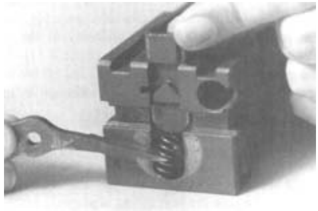
Figure 4-29. Removing and Replacing the Sear and Sear Spring.
