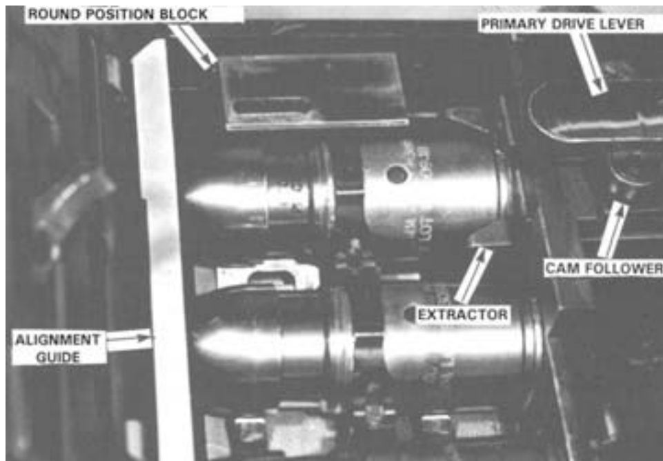
Figure 5-27. Round Positioned Against Round Positioning Block, Bolt Forward.
