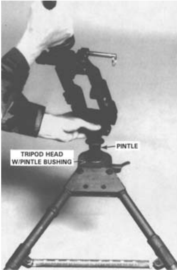
Step 1. Inserting the Pintle into Pintle Bushing.
