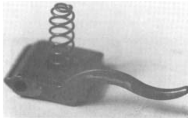
Figure 4-46. Seating the Belt Feed Pawl Spring (Left-Hand Feed).
