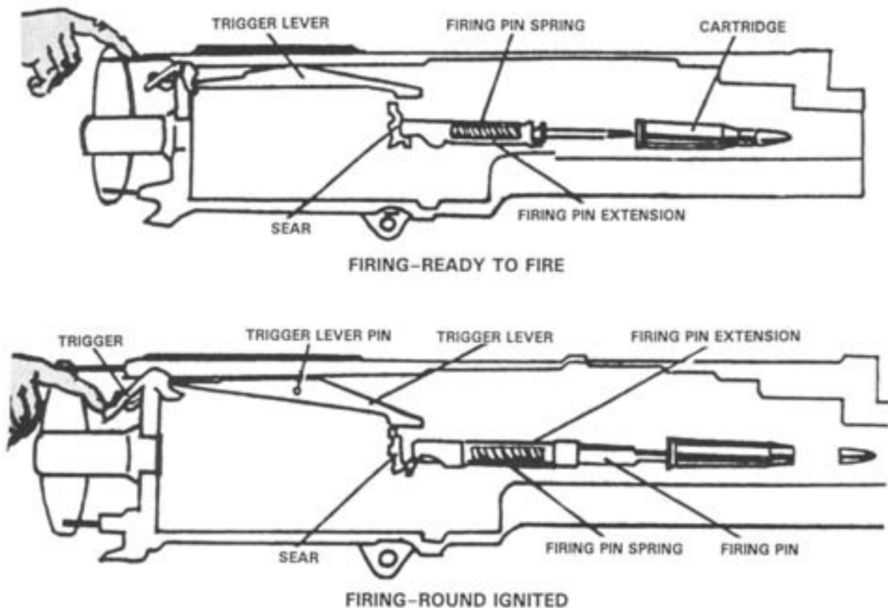
Figure 4-64. Firing.
