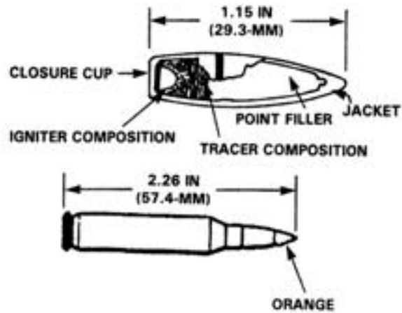
CARTRIDGE, 5.56MM, TRACER, M856
