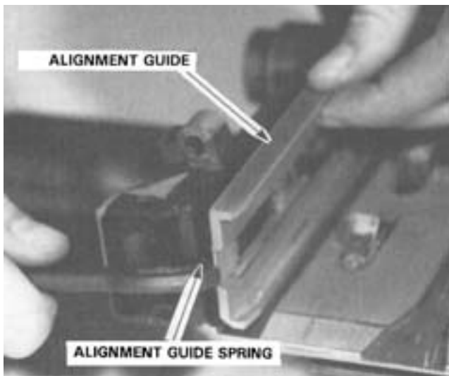
Figure 5-19. Removing the Alignment Guide Assembly.
