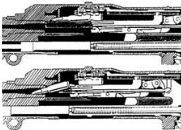
Figure 3-25. Chambering.
