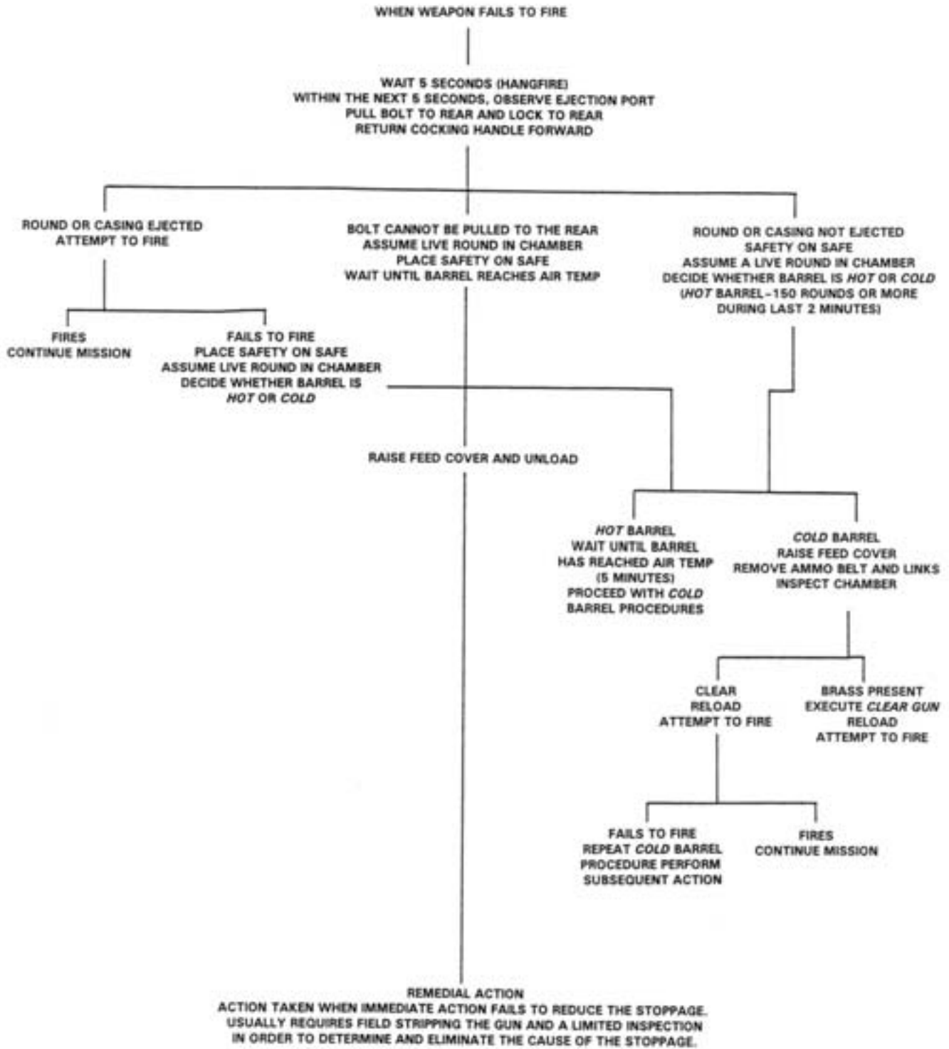
Figure 4-67. Immediate Action.
