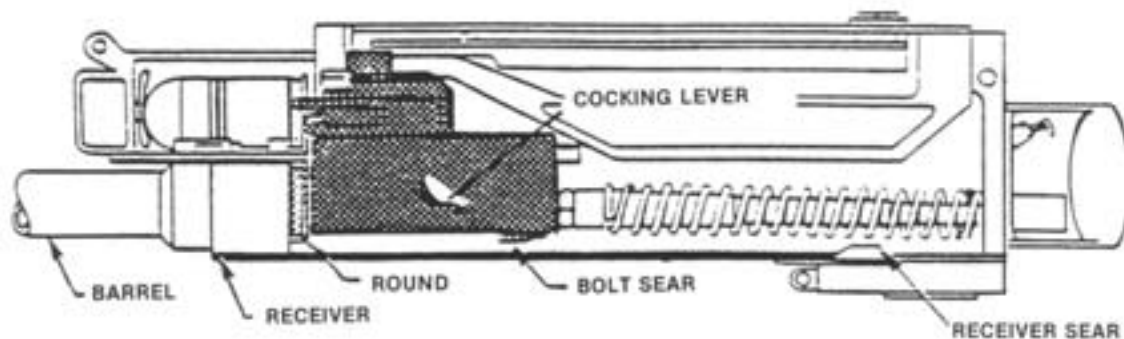
Figure 5-31. Extracting/Ejecting/Feeding/Cocking.
