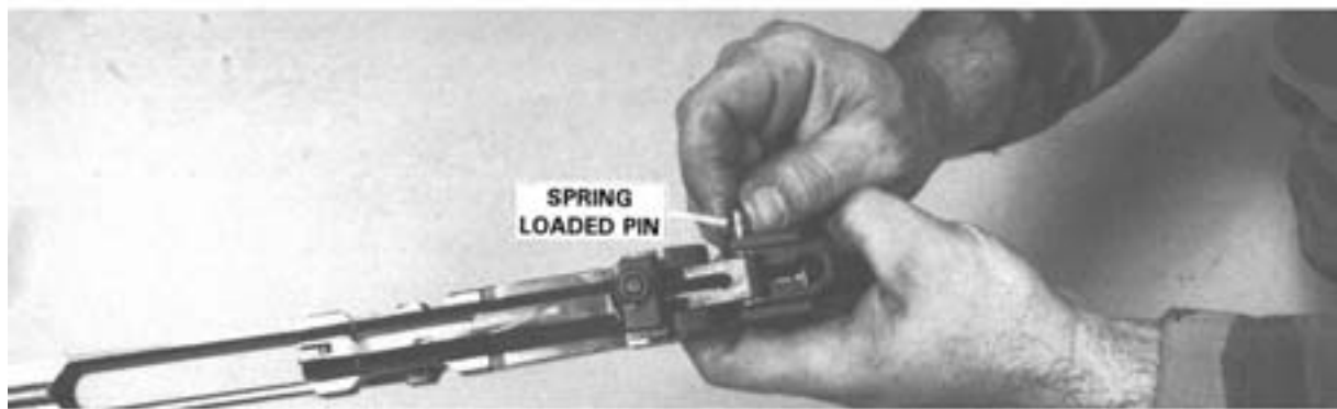
Step 2. Inserting the Spring Loaded Pin.
