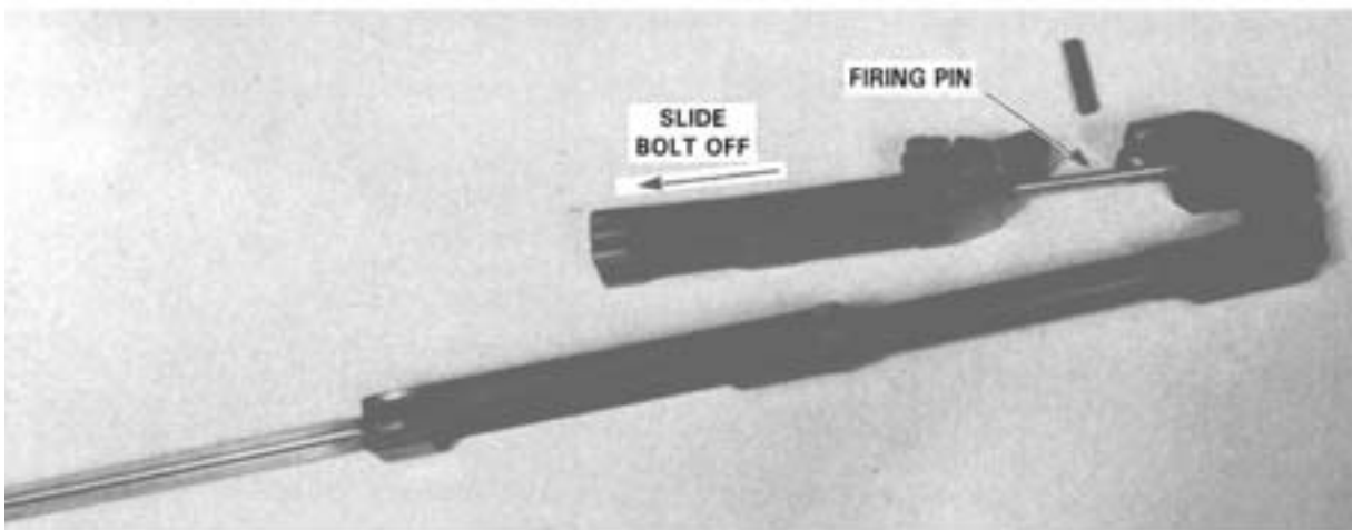
Step 2. Sliding the Bolt Forward Off Firing Pin.
