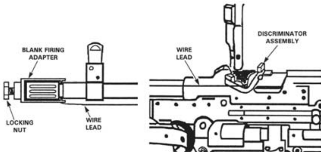
Figure 3-77. Installing the Blank Firing Adapter.
