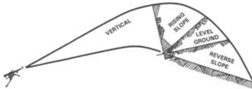
Figure 6-4. Effect of Ground Slopes on the Beaten Zone.
