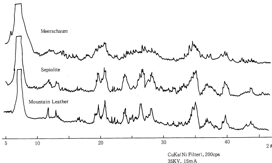
Fig. 1 X - ray diffraction patterns
