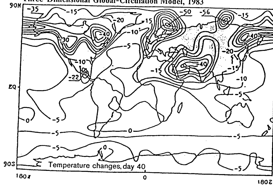
Figure 6 Soviet Nuclear Winter Research: Three-Dimensional Global-Circulation Model, 1983
