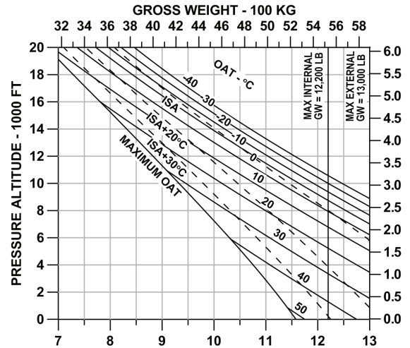
OGE All Azimuth Controllability Limitation
