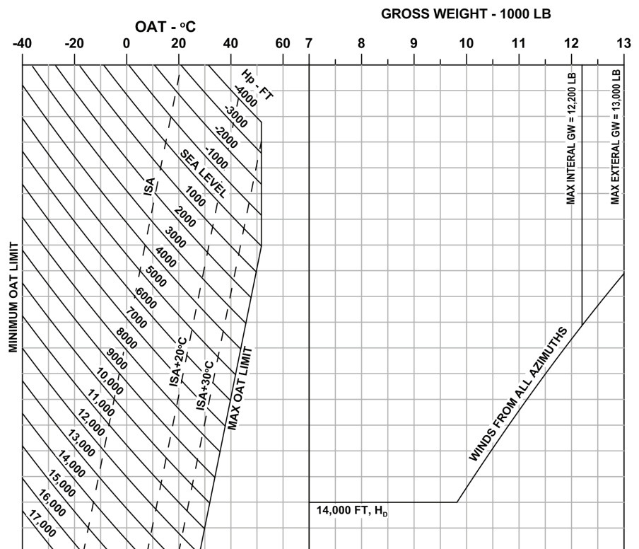
OGE All Azimuth Controllability Limitation
