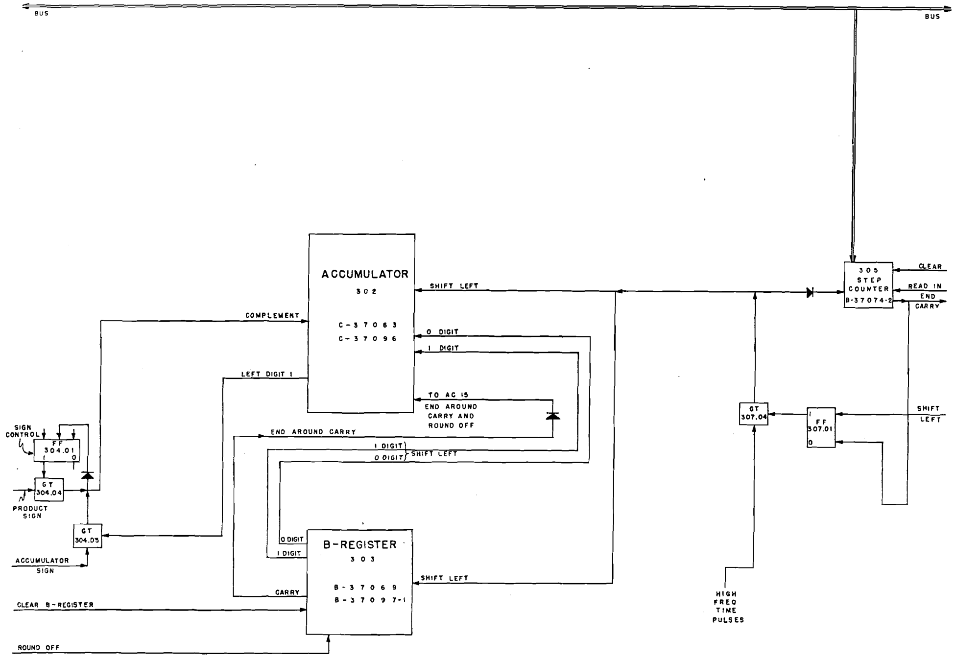
Figure 43 SHIFT LEFT
