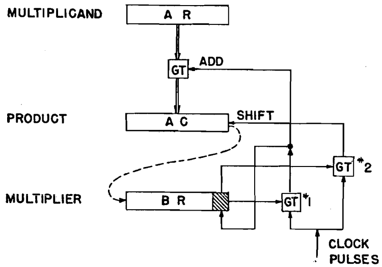
Figure 24 MULTIPLICATION IV
