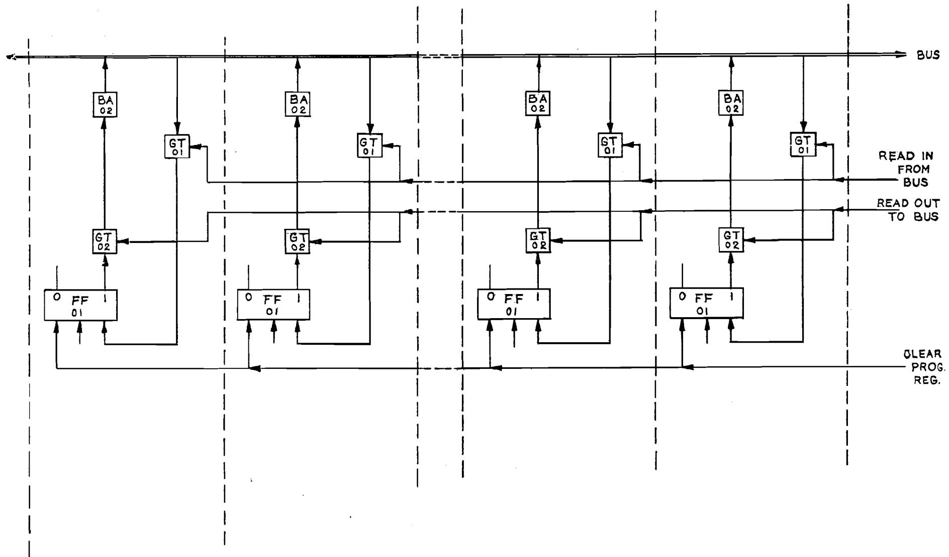
Figure 52 PROGRAM REGISTER
