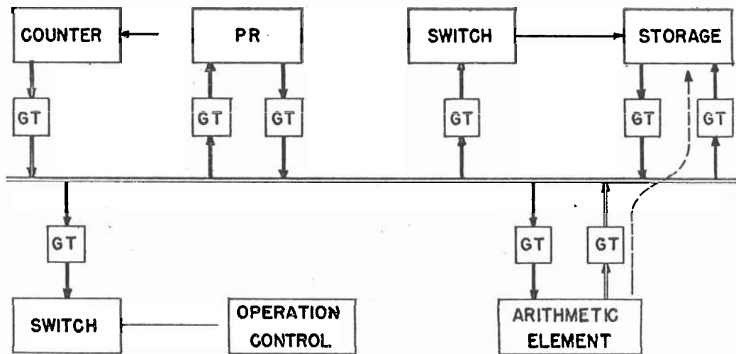
Figure 2 STORE RESULT
