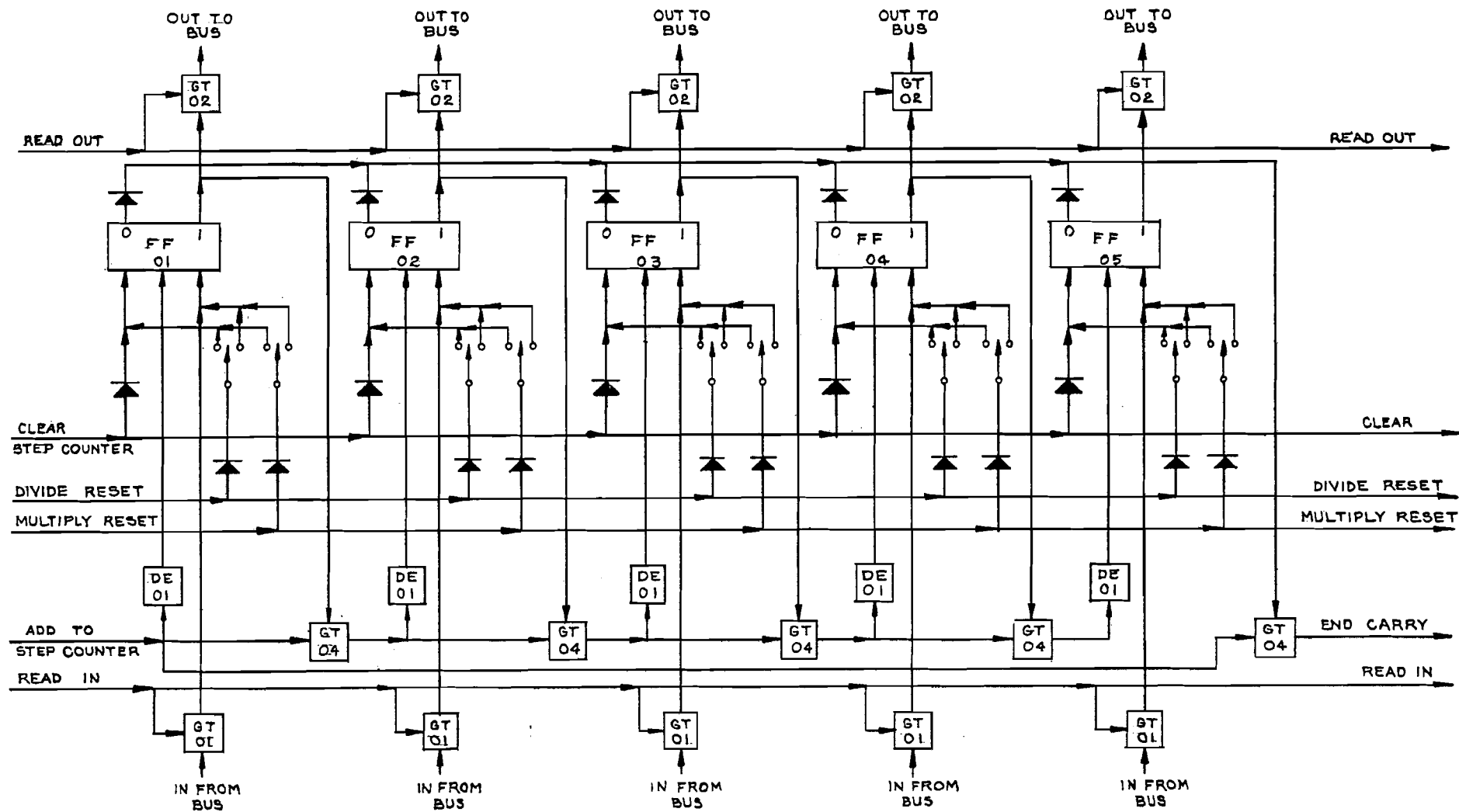
Figure 69 STEP COUNTER
