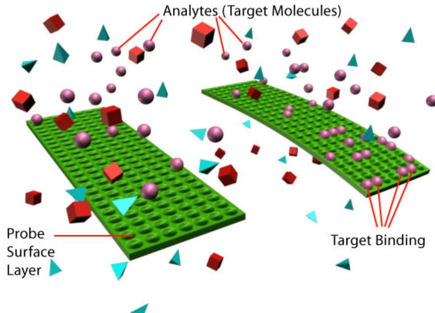
Microcantilever bending due to surface stress caused by the attachment of analytes to sensor's surface.
