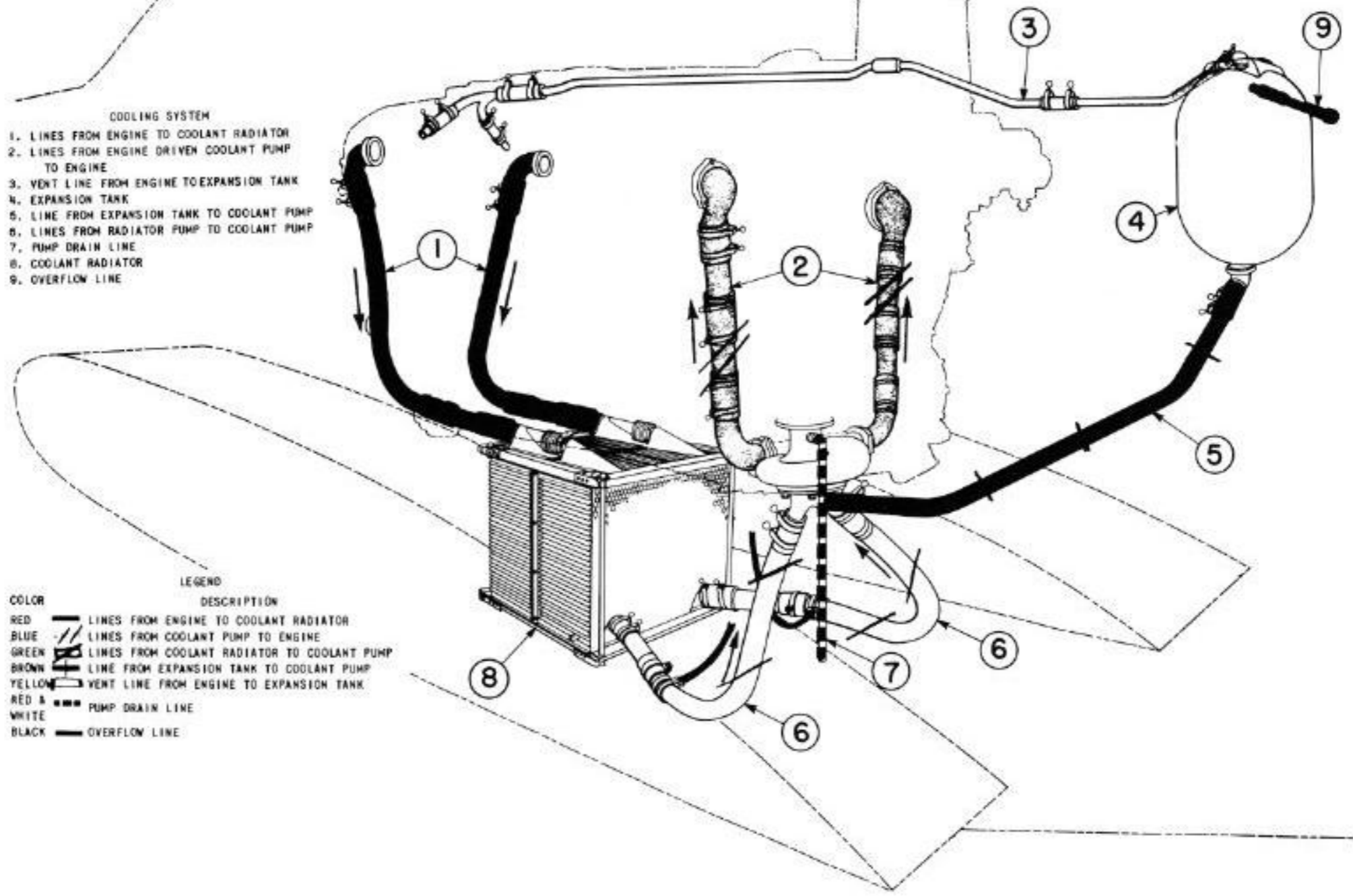
Figure 11 - Cooling System
