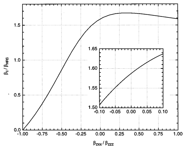
FIG. 1. The hyperpolarizability ratio, \beta_{\parallel}/\beta_{\text{HRS}} , as calculated from Eqs. (3) and (6) for HRS measurements in the VV polarization geometry, as a function of the value of R = \beta_{zxx}/\beta_{zzz} for C_{\infty v} symmetry. The inset shows the relation between the hyperpolarizability ratio \beta_{\parallel}/\beta_{\text{HRS}} and values of R in an expanded scale near R = 0 .
