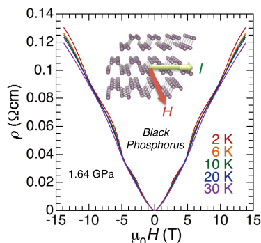
Magnetoresistance of a single crystal of black phosphorus under multiple extreme conditions. Inset shows schematic illustration of the crystal structure. Resistance along the c axis was measured in magnetic fields applied along the a axis. We observed huge positive magnetoresistance larger than 1,000 times of the value at zero field together with superposed Shubnikov-de Haas oscillations.
