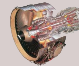
CFM56-5B
