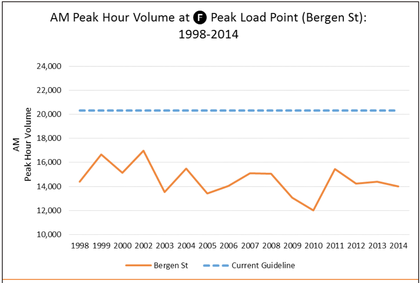
Figure 5- F Line Peak Hour Load Trend
