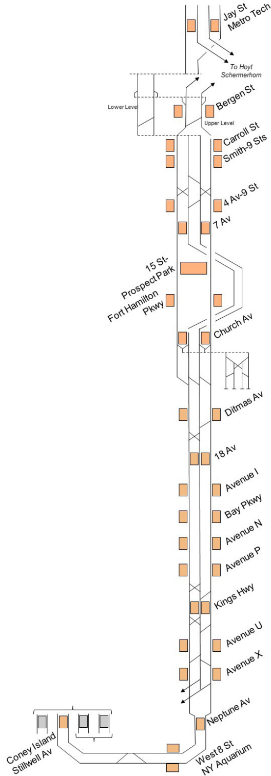
Figure 1-Culver Line Track Configuration
