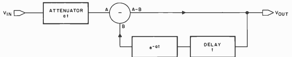
Figure 7: Filtering process performed by the circuit of figure 6 in block form. By changing a sum to a difference we convert the block diagram from a low to a high pass filter.
