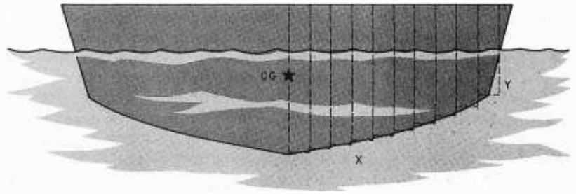
Figure 3: The continuous hull of a boat can be divided into a series of discrete segments or "bottles." X is the distance from the center of gravity to the center of the bottle. Y is the length of the bottle below the water line at equilibrium. Note that the symmetry about the CG enables us to describe the hull while only segmenting half of it.
