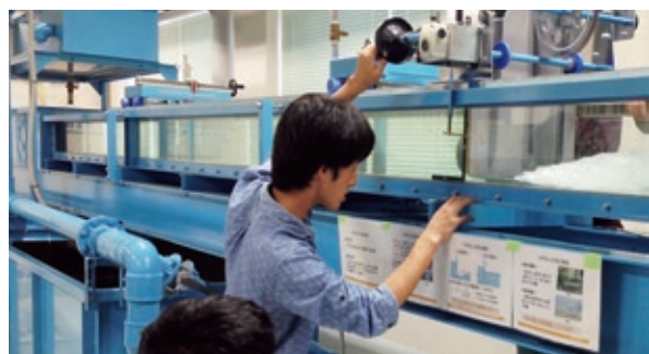
▲ 開水路実験 Experiments Using Open Channel
