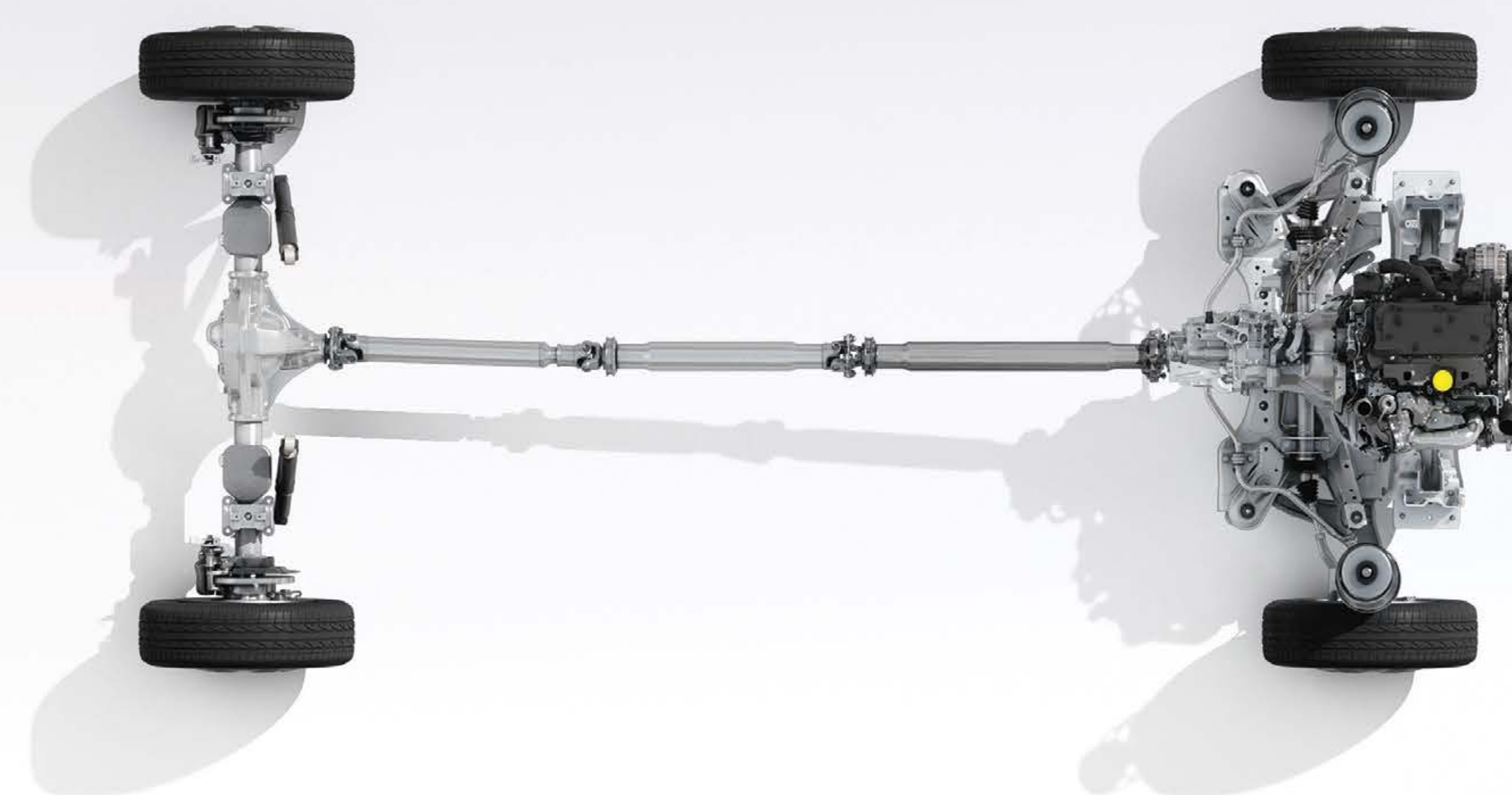
rear-wheel drive
