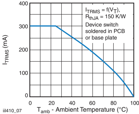
Fig. 5 - Current Reduction
