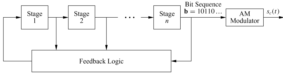
Figure 13.6: Generation of spreading codes.
