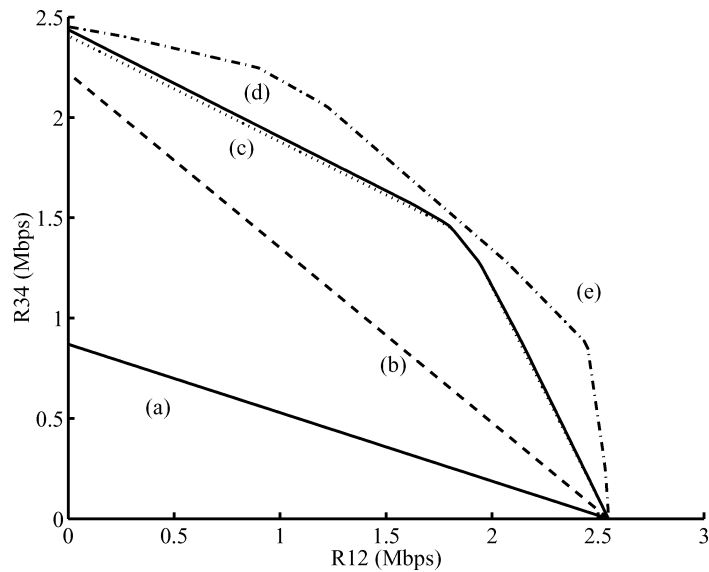
Figure 16.4: Capacity region slice of five-node network along the plane R_{ij} = 0 , where \{ij\} \neq \{12\}, \{34\} and i \neq j . (a) Single-hop routing, no spatial reuse. (b) Multihop routing, no spatial reuse. (c) Multihop routing with spatial reuse. (d) Two-level power control added to (c). (e) Successive interference cancellation added to (c).
