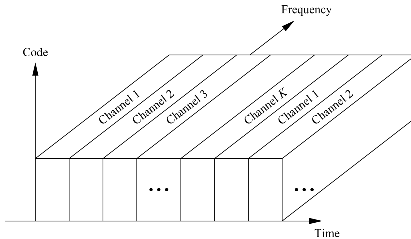
Figure 14.3: Time-division multiple access.
