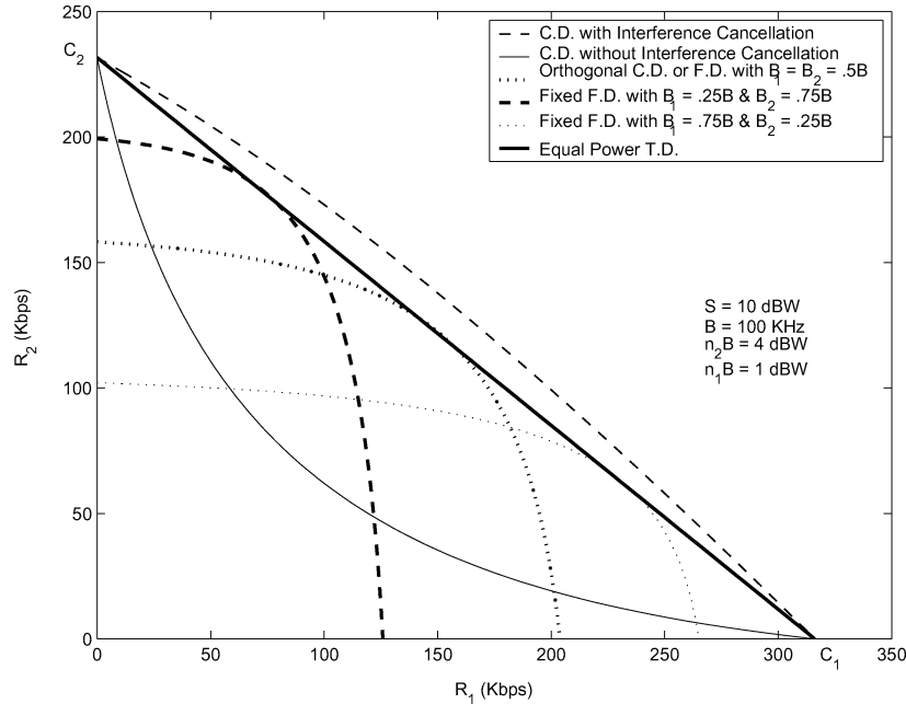
Figure 14.10: Two-user capacity region with 3-dB SNR difference.
