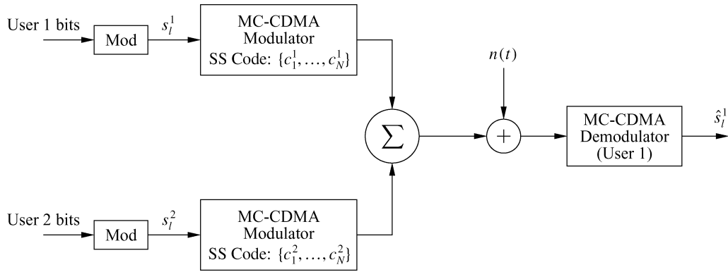
Figure 13.18: Two-user multicarrier CDMA system.
