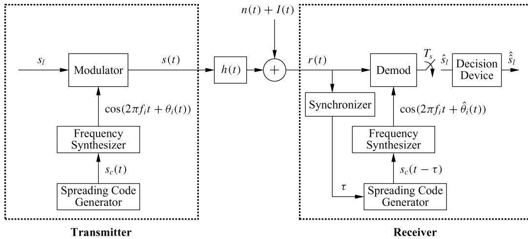
Figure 13.11: FHSS system model.
