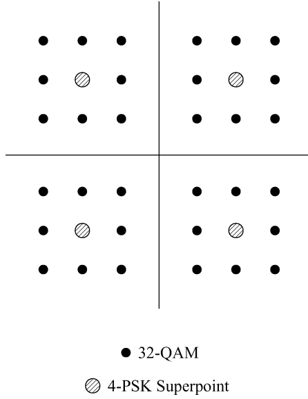
Figure 14.9: 32-QAM with embedded 4-PSK.
