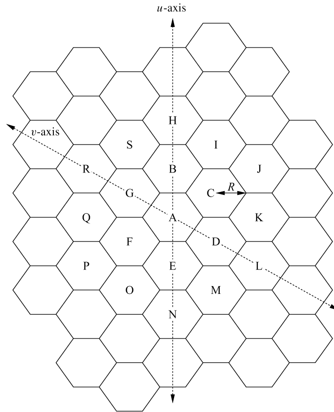
Figure 15.4: Axes for reuse distance in hexagonal cells.
