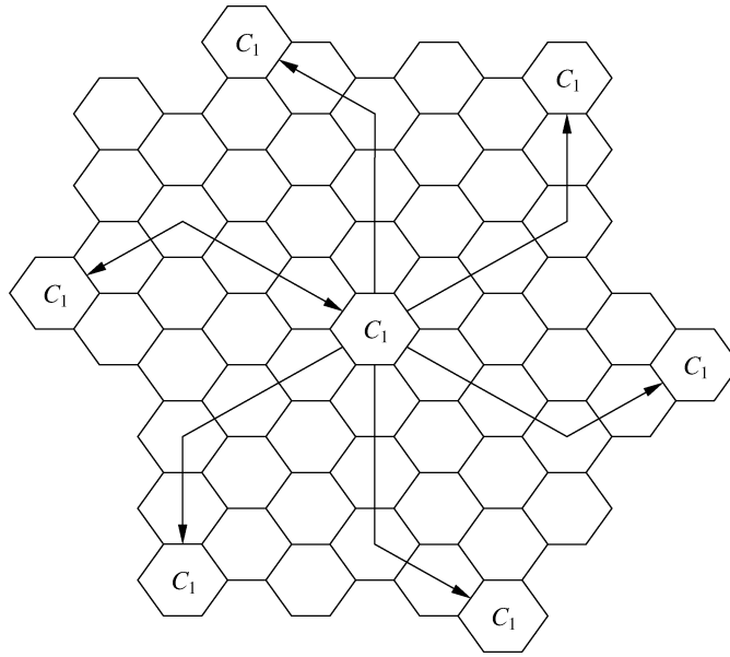
Figure 15.6: Channel assignment in hexagonal cells.
