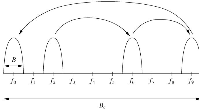
Figure 13.4: Frequency hopping.
