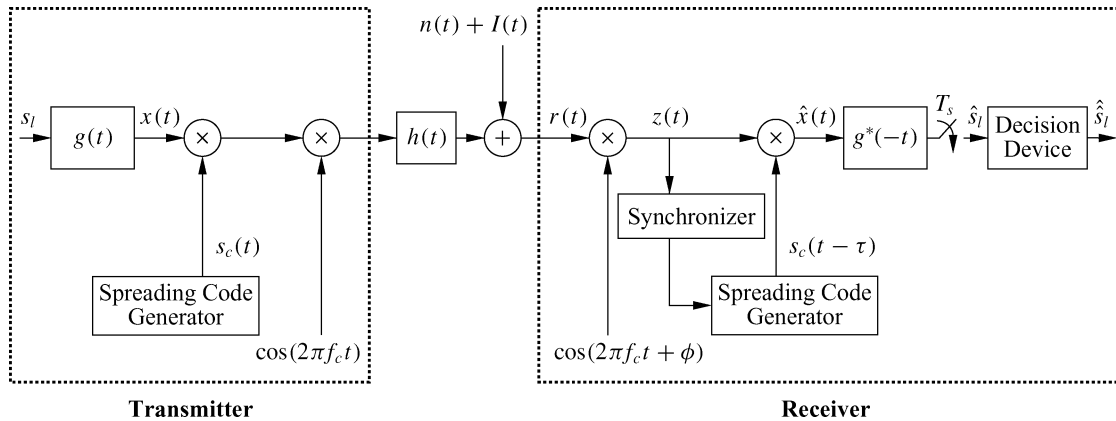
Figure 13.5: DSSS system model.
