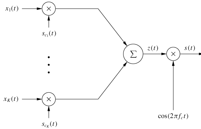
Figure 13.13: Downlink transmitter.
