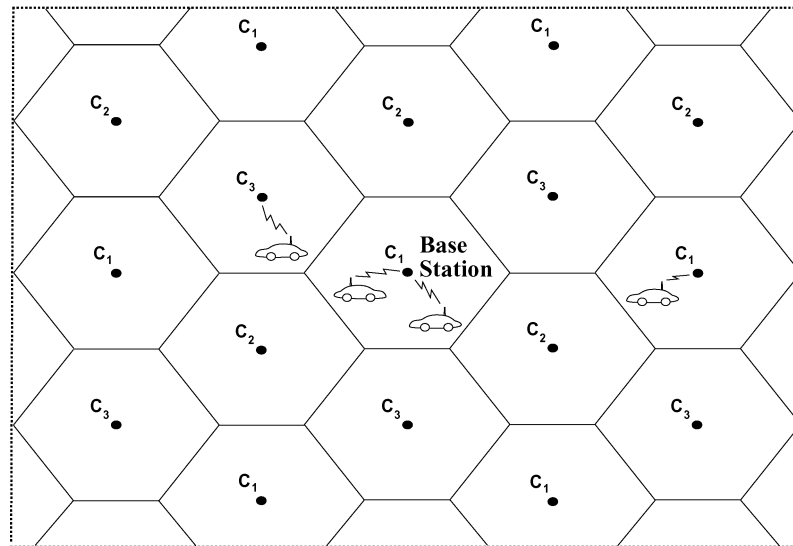
Figure 15.1: Cellular system.
