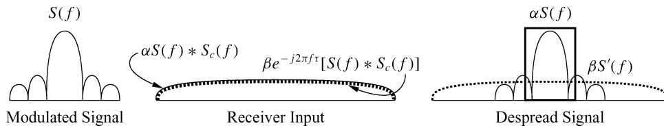
Figure 13.3: ISI rejection in DSSS.
