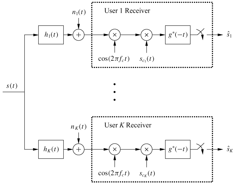
Figure 13.14: Downlink channel and receiver.
