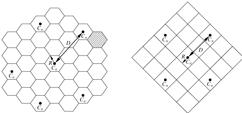
Figure 15.3: Reuse distance D with a given reuse pattern for hexagonal and diamond-shaped cells.
