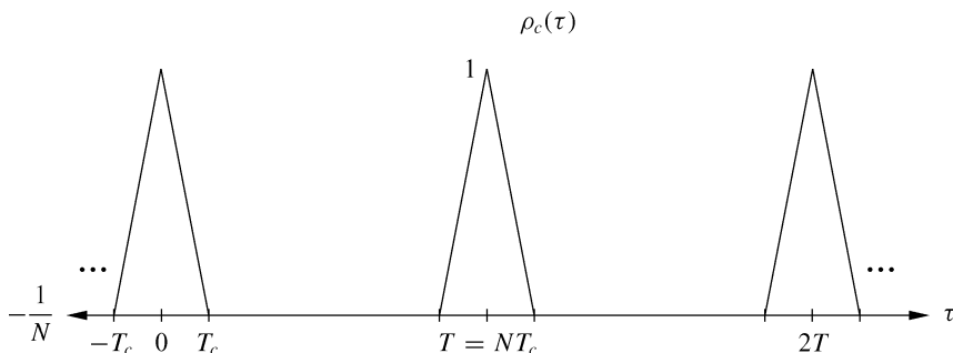
Figure 13.8: Autocorrelation has period T = NT_c .
