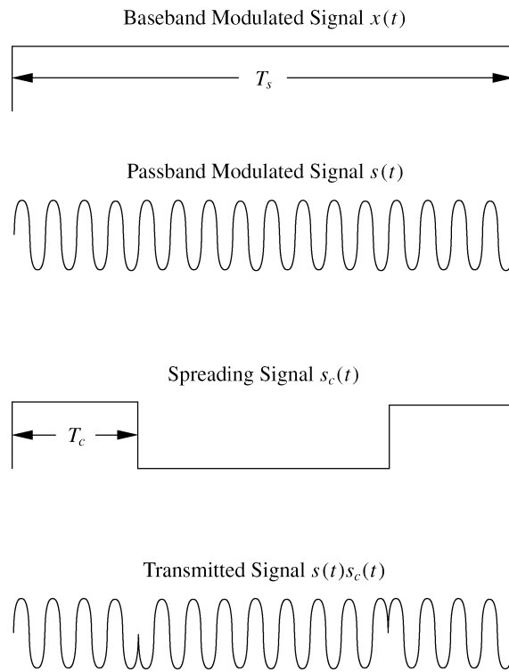
Figure 13.1: Spreading signal multiplication.
