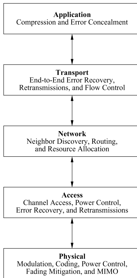
Figure 16.2: Five-layer model for network protocol design.
