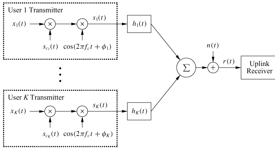
Figure 13.15: DSSS uplink system.
