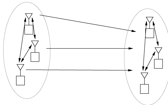
Figure 16.5: Cooperative MIMO.
