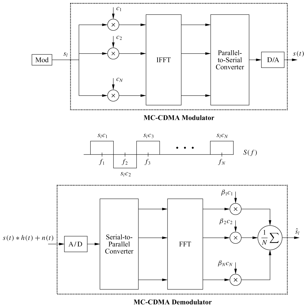
Figure 13.17: Multicarrier CDMA system.
