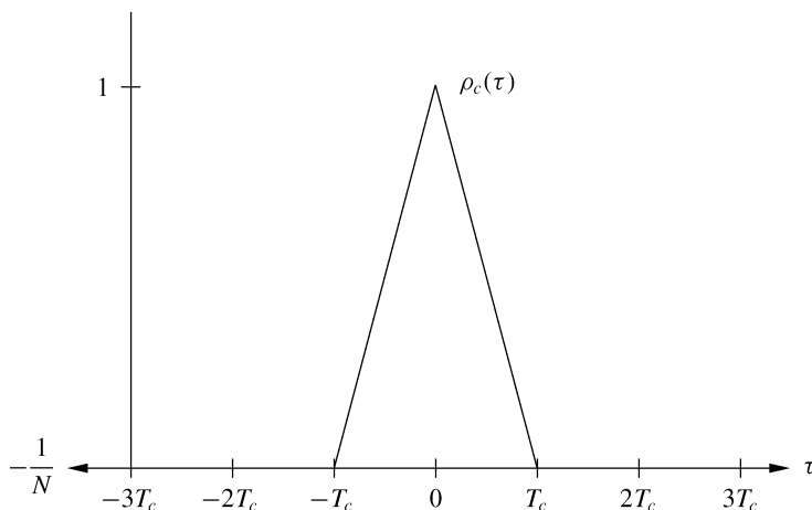
Figure 13.7: Autocorrelation of maximal linear code ( N = T/T_c ).
