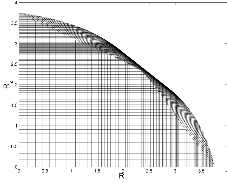
Figure 14.13: MIMO BC capacity region with \mathbf{H}_1 = [1 \ 0.5] , \mathbf{H}_2 = [0.5 \ 1] , and P = 10 .
