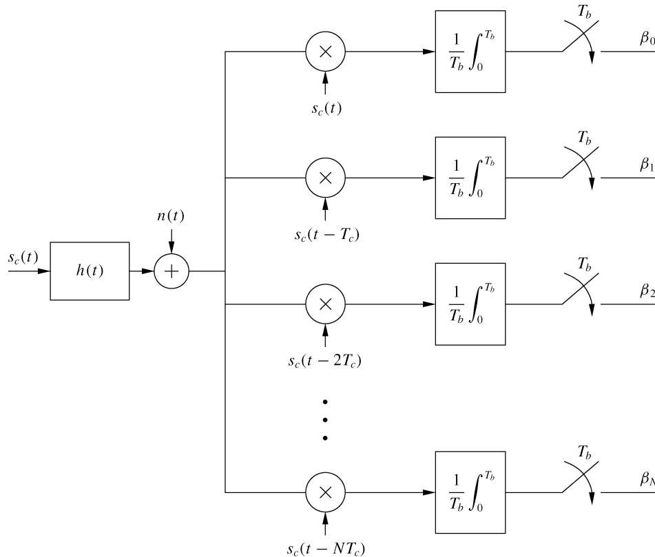
Figure 13.19: Channel sounder for Problem 13-15.
