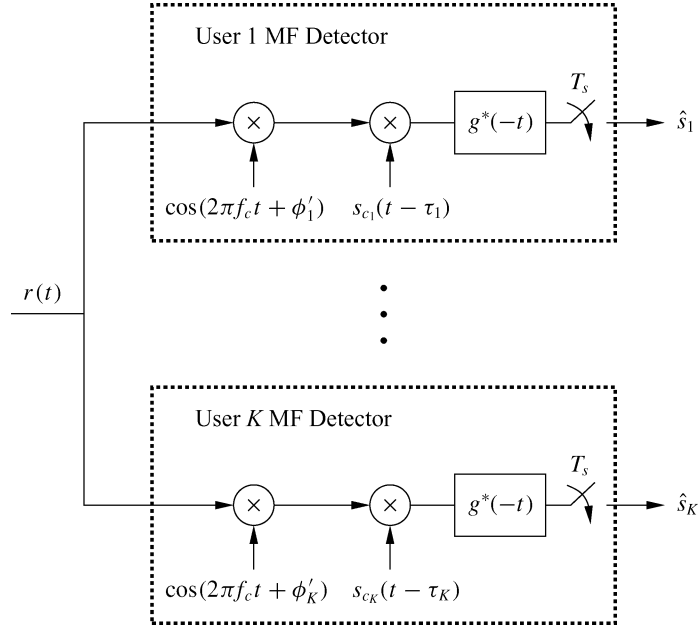
Figure 13.16: Uplink receiver.
