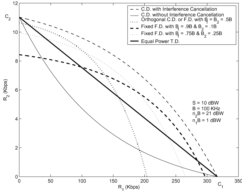
Figure 14.11: Two-user capacity region with 20-dB SNR difference.
