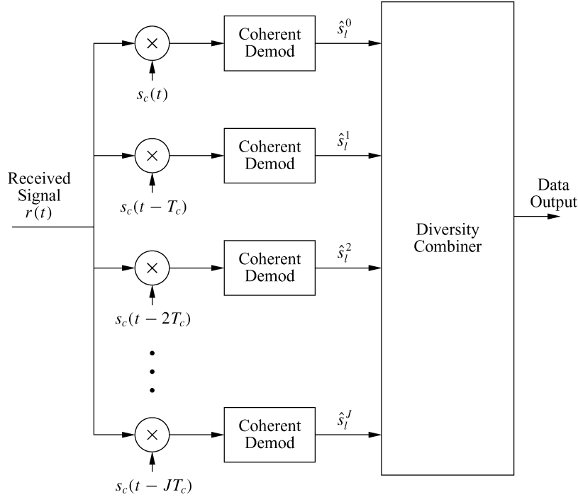
Figure 13.10: RAKE receiver.
