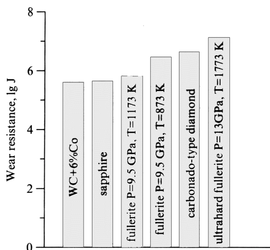
Fig. 4. Results of the wear tests of specimens of hard alloy WC + 6%Co, sapphire, carbonado-type diamond, super- and ultrahard fullerites (synthesis conditions are mentioned in the figure)
