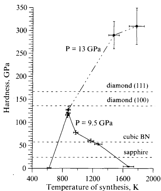
Fig. 3. Results of the hardness tests of fullerite specimens. The hardness values are plotted vs temperature of synthesis. The specimens were synthesized at pressure 9.5 and 13 GPa. Hardness levels of sapphire, cubic BN and diamond are plotted for comparison.
