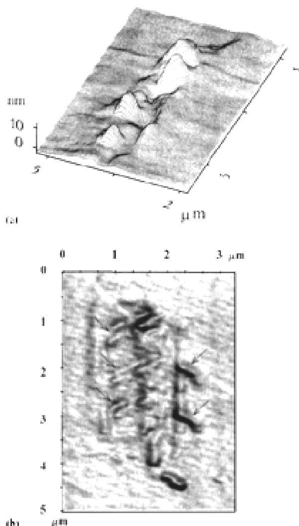
Fig. 2. The NanoScan images of the scratches of the sclerometry tests obtained with the ultrahard fullerite tip on the (111) diamond face (a); and with the diamond tip on the (111) diamond face (b). Cracks are marked by arrows, vertical scale is 2 nm for (b).
