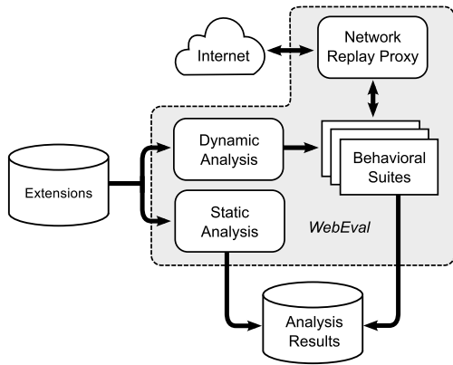
Figure 4: WebEval’s analysis pipeline for scanning Chrome Web Store extensions.
