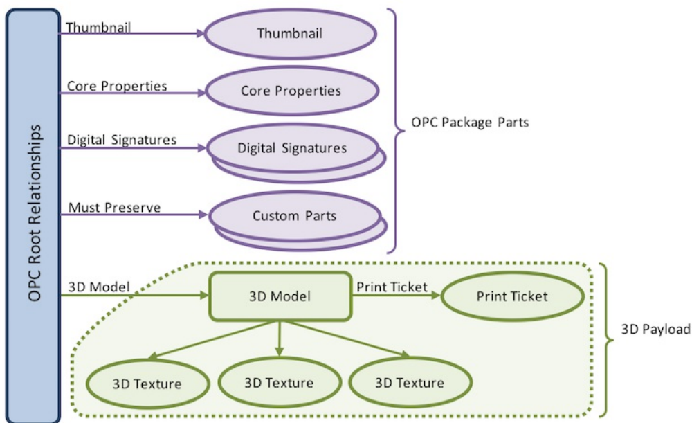
Figure 2-1. A typical 3MF Document
