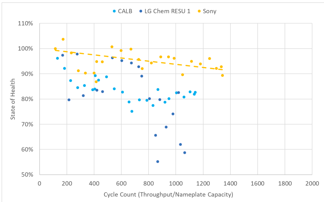
Figure 3 Average capacity fade results for Phase 1 Batteries
