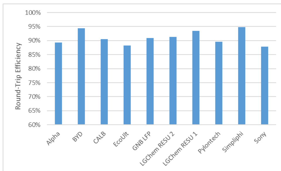
Figure 5. Average round-trip efficiency of various battery packs
