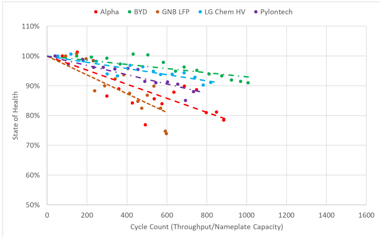
Figure 4 Average capacity fade results for Phase 2 Batteries
