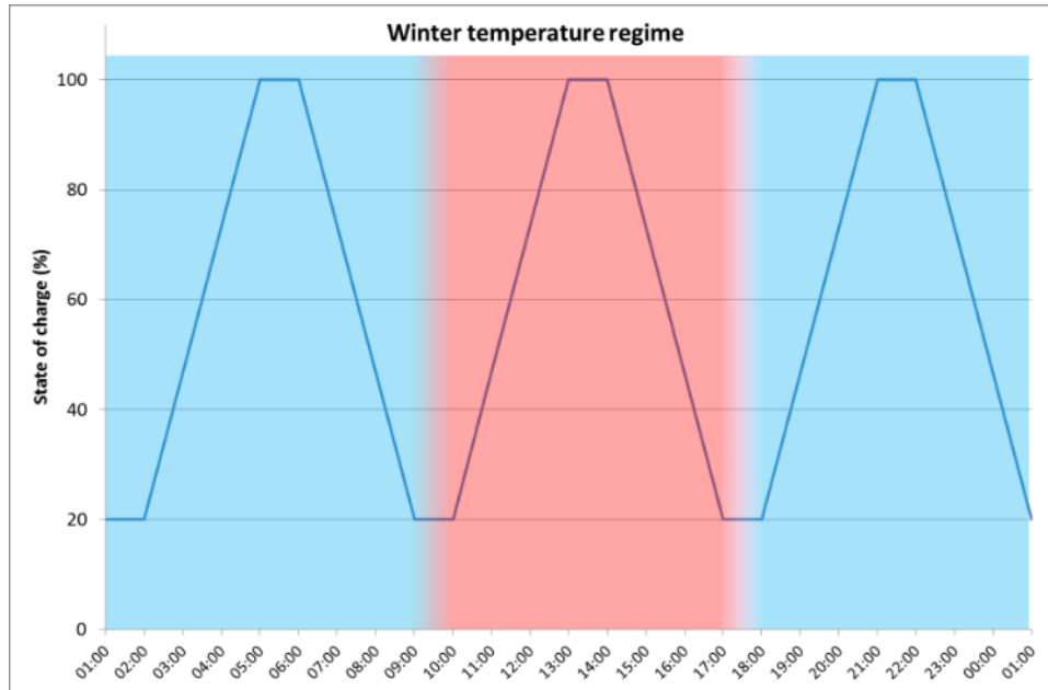
Figure 11: Winter temperature regime and charge regime
