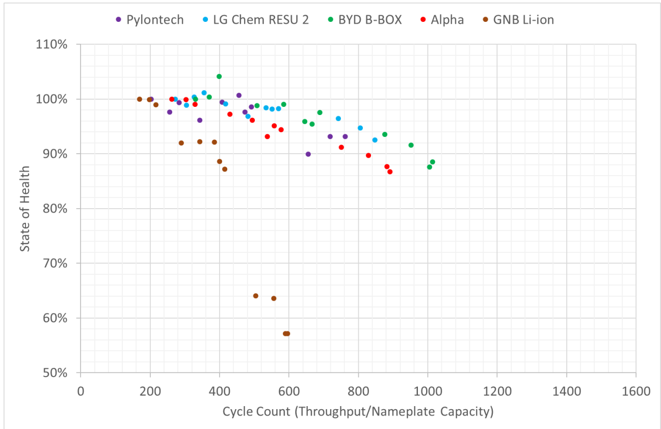
Figure 2. Capacity fade of Phase 2 battery packs
