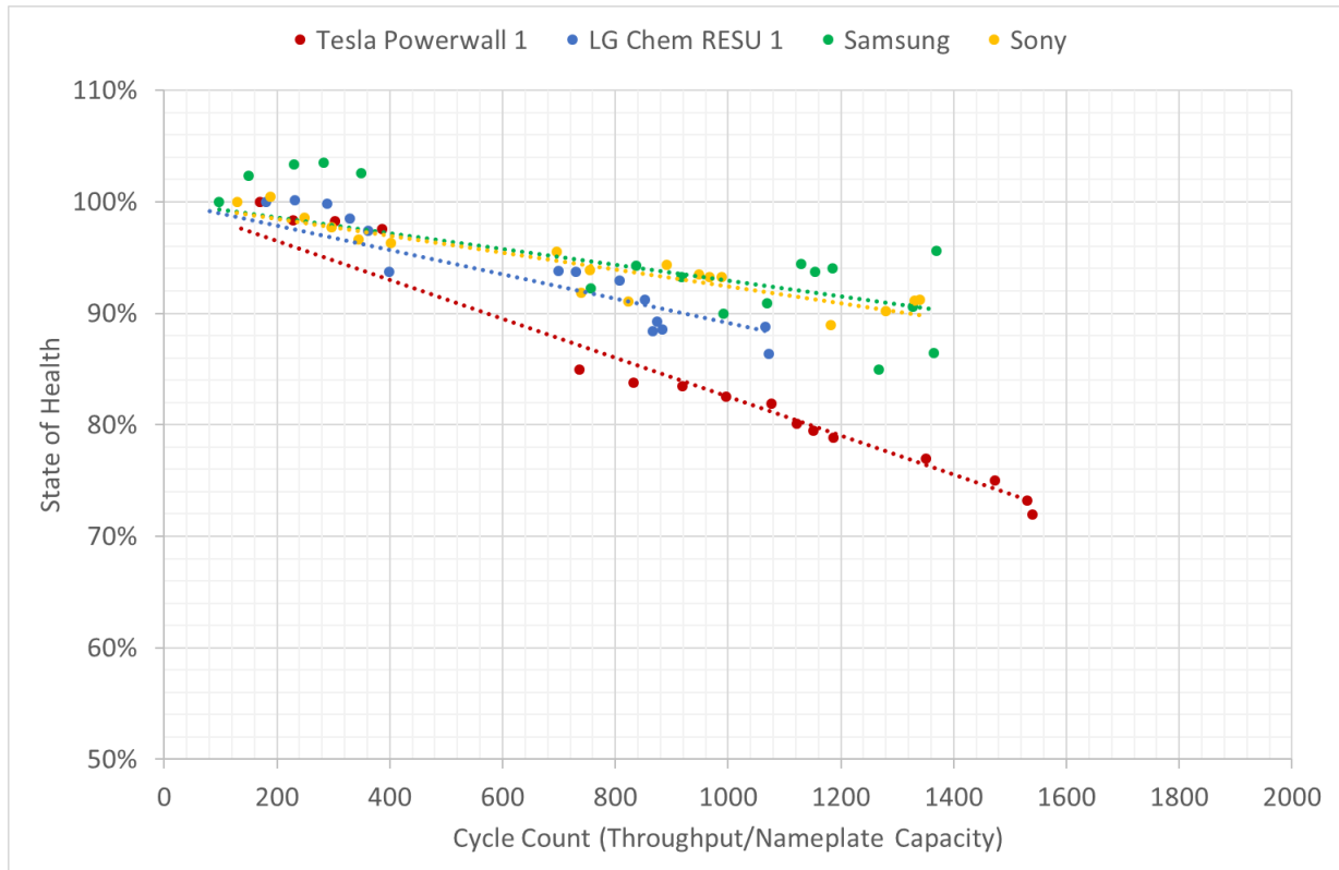
Figure 1. Capacity fade of Phase 1 battery packs based on monthly capacity tests
