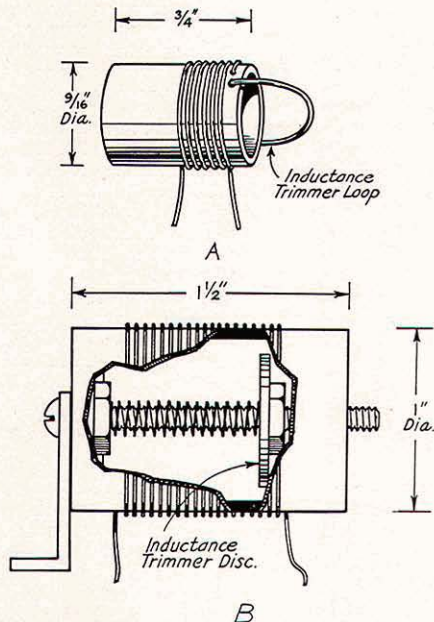
FIG. 1—INDUCTANCE TRIMMING METHODS
