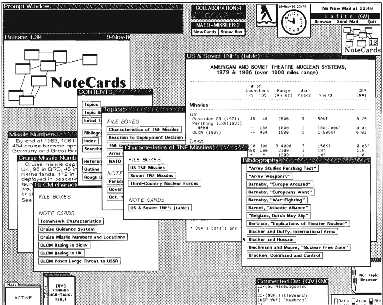
Figure 7. A typical NoteCards screen with five FileBox cards, two unformatted Text cards, and one Text card formatted as a table. Links between cards are represented by the boxed text inside the cards. The two menus at the top/middle of the screen control two different note files. The remainder of the icons on the screen belong to non-NoteCard applications running in the Xerox Lisp environment.
