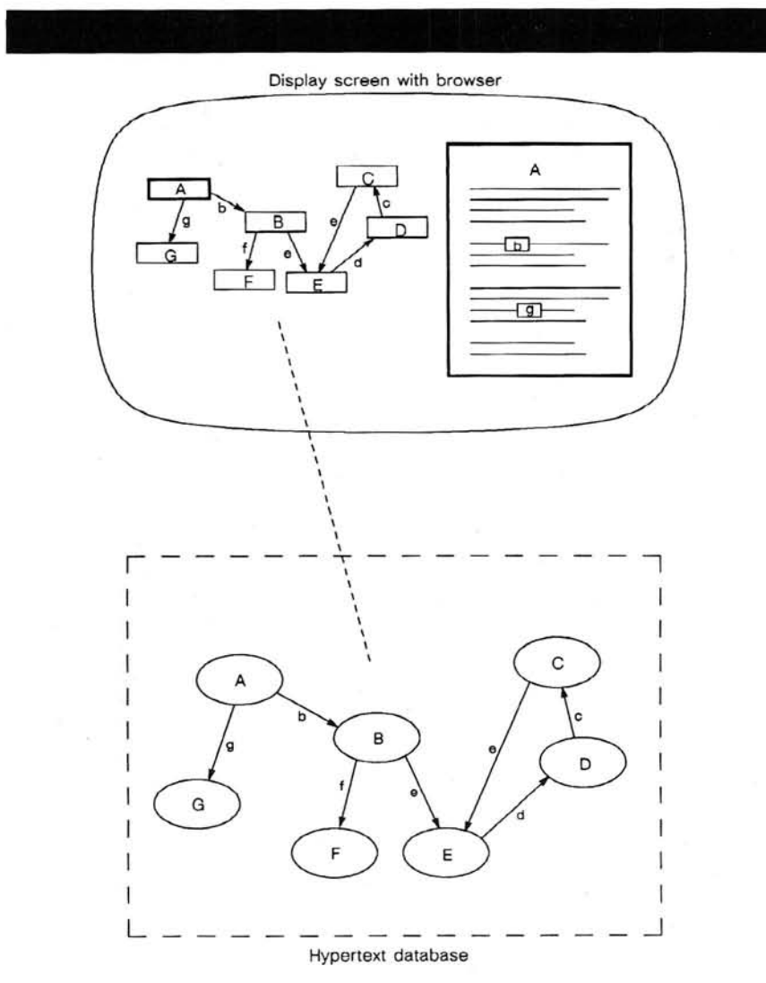
Figure 2. The screen at the top illustrates how a hypertext browser provides a direct two-dimensional graphic view of the underlying database. In this illustration, the node "A" has been selected for full display of its contents. Notice that in the browser view you can tell not only which nodes are linked to A but also how the subnetwork fits into the larger hyperdocument. (Of course, hyperdocuments of any size cannot be shown all at once in a browser—only portions can be displayed.)
