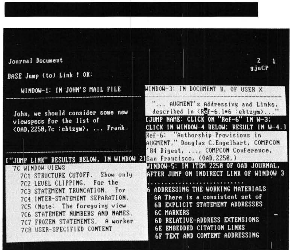
Figure 4. Augment display showing five windows. Window 1 (W-1) has a passage as if embedded in a message, showing a link to Branch 7c of Document 2250 in the OAD Journal. A ViewSpec ("ebtzgm") provides the following specifications: target level plus one, truncate to one line per statement, no blank lines between statements, show only that branch (e.g., not Branch 7d), and turn on Location Numbers. Window 2 (W-2) shows the view obtained with a jump link command. To perform a jump link command, the operator clicks on the link in W-1, then moves the cursor into W-2 for the final click. The very top-left system message announces that the desired Journal Item has been accessed, and the cluster at the top left of the screen verifies that the view is clipped to three levels and the statements truncated to one line each. Window 3 (W-3) shows an indirect link that specifies the linkage path. In effect, this link says "go to the statement in the file named 'Ref-6,' follow the link found there to its target file, and in that file find Location Number 6." Note that the same ViewSpec is specified here as for the link in W-1. Window 4 (W-4) identifies Ref-6 and provides its general reference source as the reference section at the end of the document; a user can jump from the link citation in W-3 to see this statement by using the jump name command. To perform this command, he clicks on "Ref-6" in W-3 then clicks on W-4. Window 5 (W-5) shows a view in the OAD-Journal Item 2250. The user can obtain this view by performing a jump link command on the indirect link of W-3. To perform this command, the user clicks on the indirect link of W-3 and then clicks in W-5.
