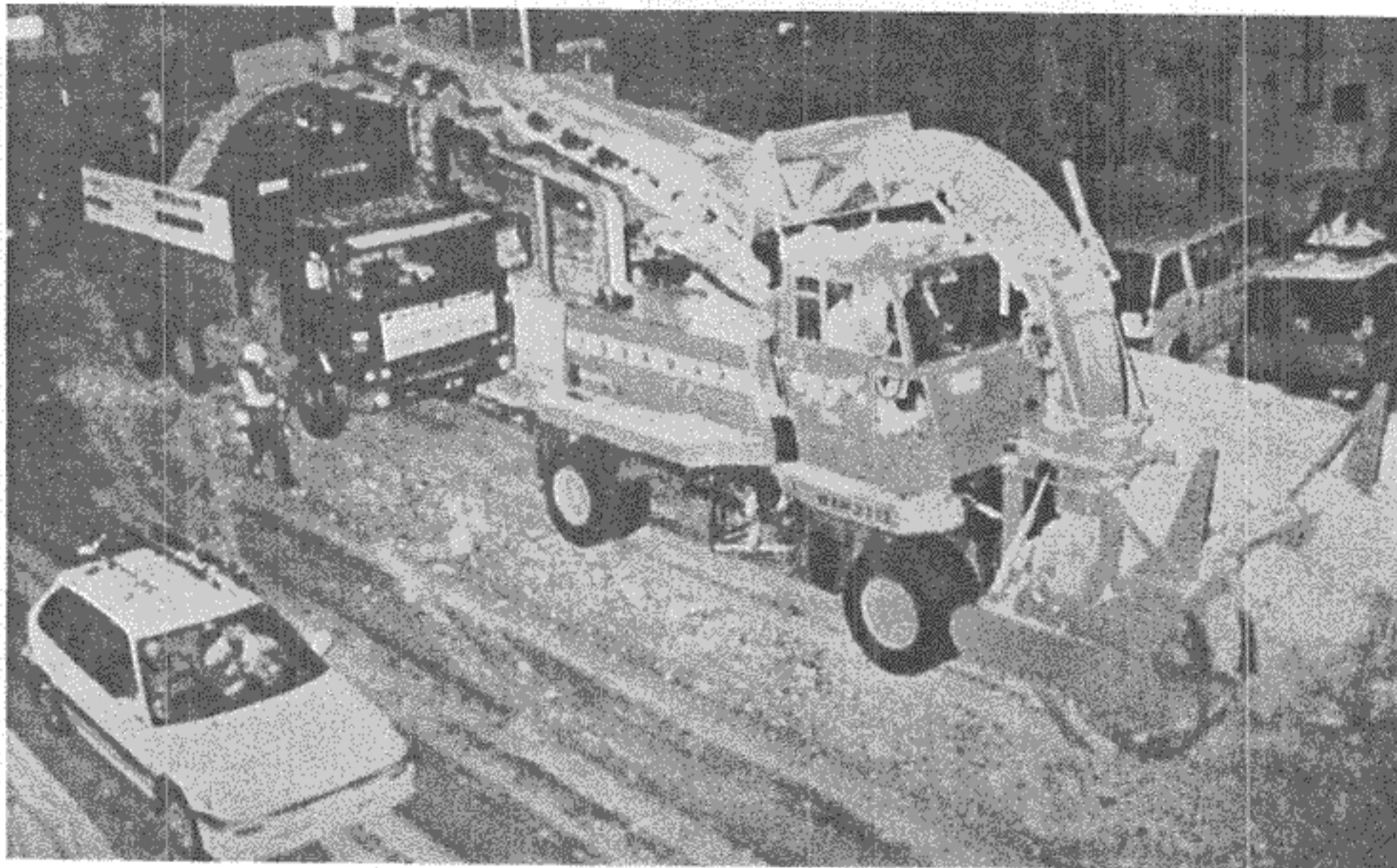
Figure 2. Single-lane-obstructing rotary snow plow.
