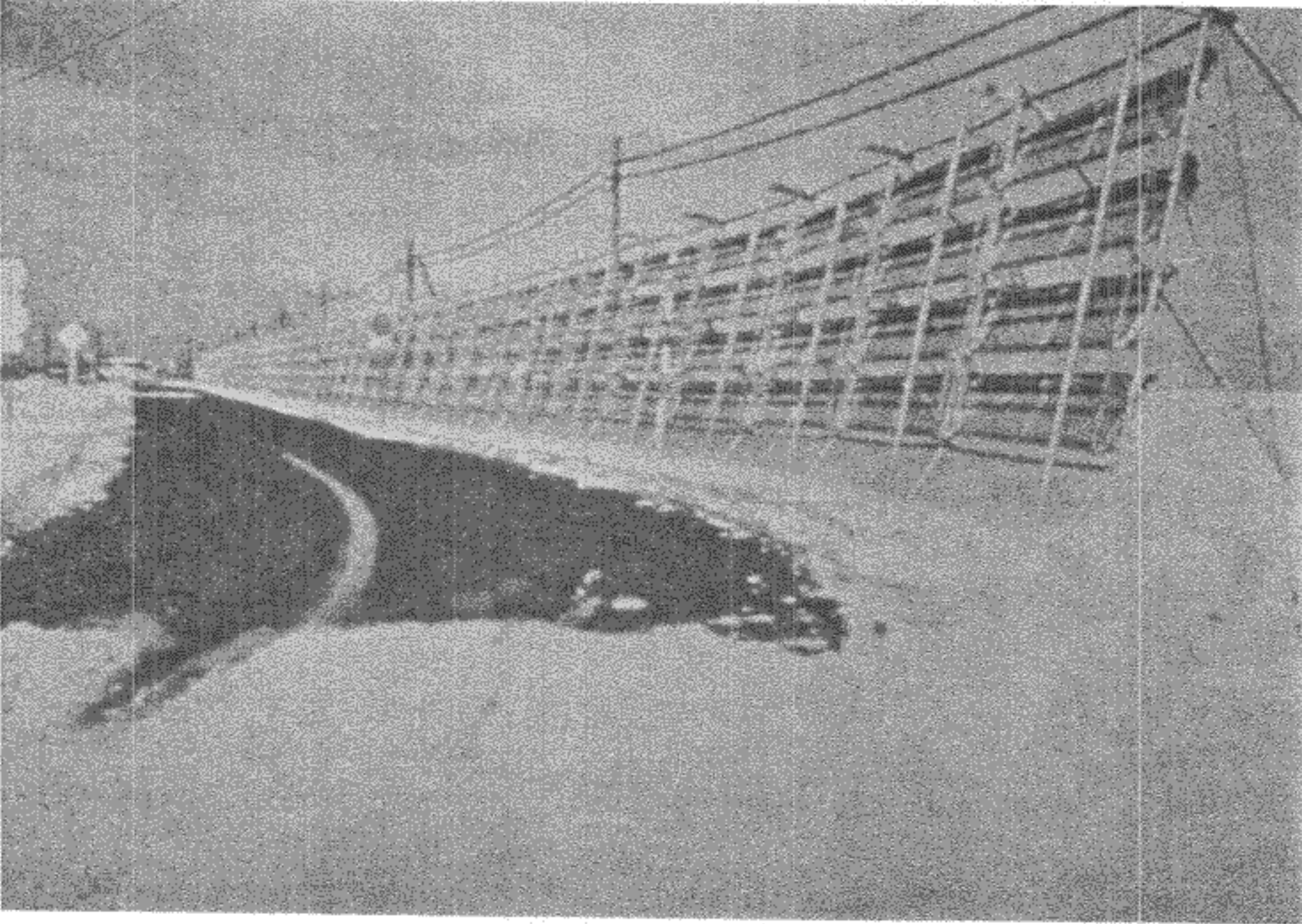
Figure 5. Blower-type fence.
