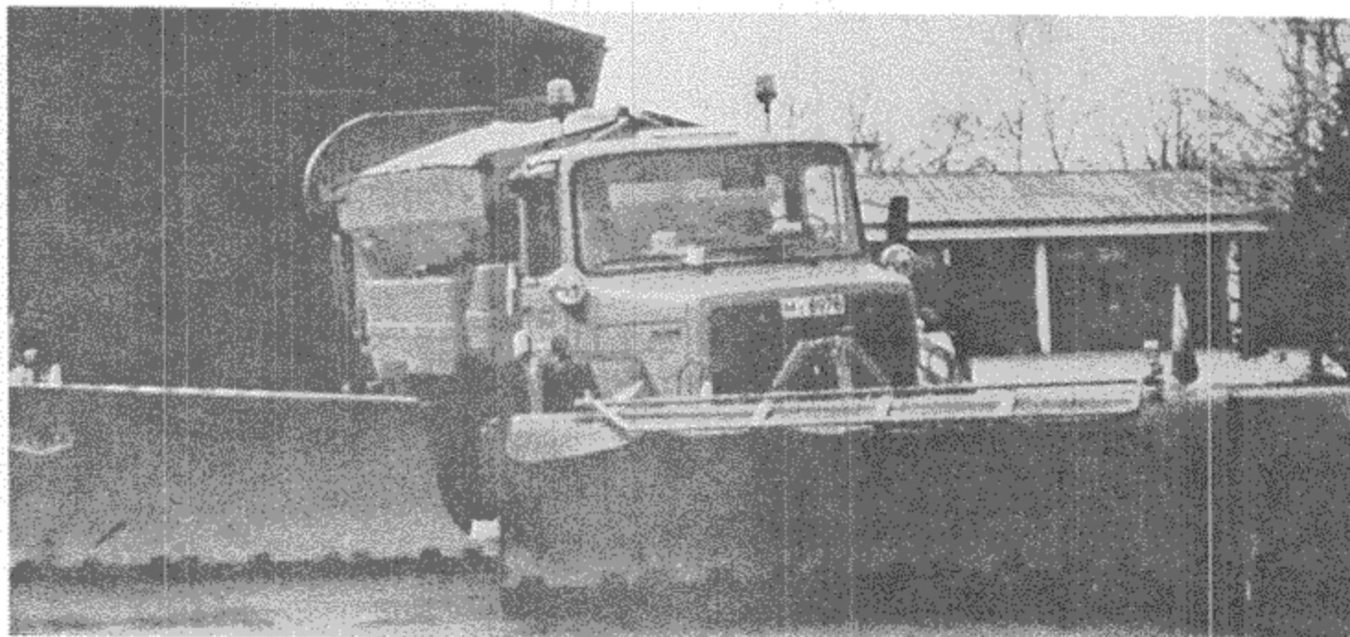
Figure 3. Sectional plow.
