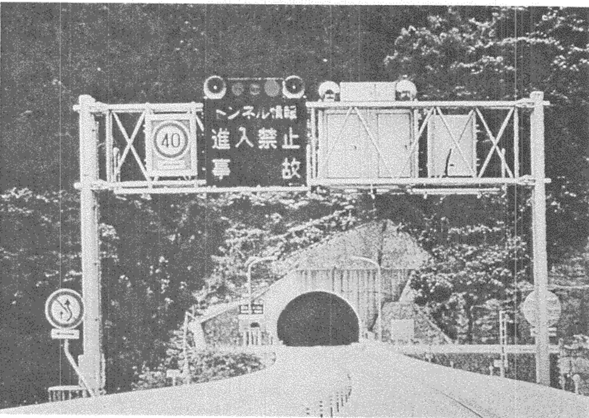
Figure 6. Variable speed limit system.
