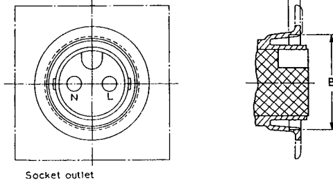
Socket outlet
